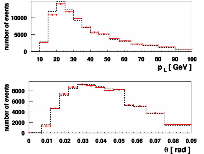
FIG. 4. The distributions of the longitudinal momentum and the scattering angle for the hadron with the highest p_T . The points correspond to the proton data from 1993 and the histograms to the Monte Carlo simulation with the modified fragmentation function.
