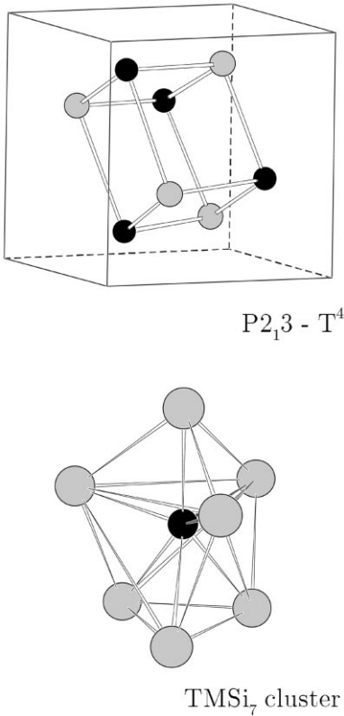
Fig. 1. Crystal structure with the T^4 - P2_13 space group, and a TMSi_7 cluster representing the site symmetry of individual atoms in this structure.
