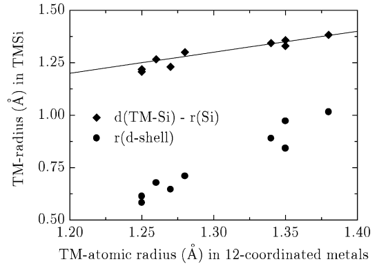
Fig. 2. TM radius in TM-Si (TM-Si bondlength minus radius of Si, diamonds) and d-shell radii (circles) versus the TM radius in 12-coordinated metals.
