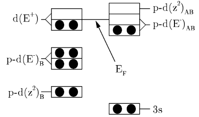
Fig. 8. Schematic diagram of the energy levels in TMSi. The situation with two electrons in the d(E^+) level which is displayed here corresponds to FeSi.
