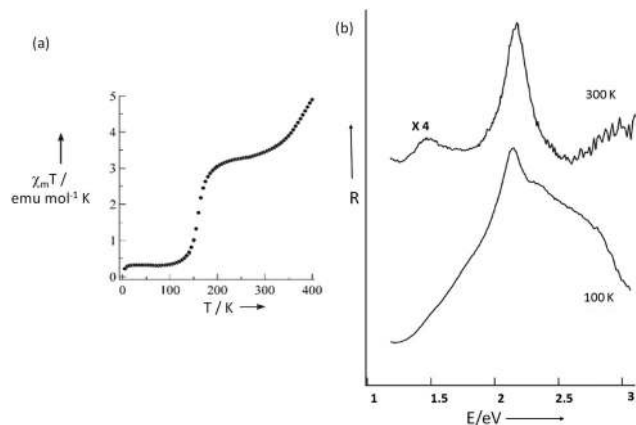
Fig. 32 (a) Plot of \chi_m T vs. T for [\text{Fe}_2\text{L35}(\text{L48})_2(\mu\text{-CN})_2](\text{PF}_6)_4 ; (b) reflectance spectra; R = reflectivity, E = photon energy. Figure adapted with permission from ref. 122. Copyright 2005 John Wiley and Sons.
