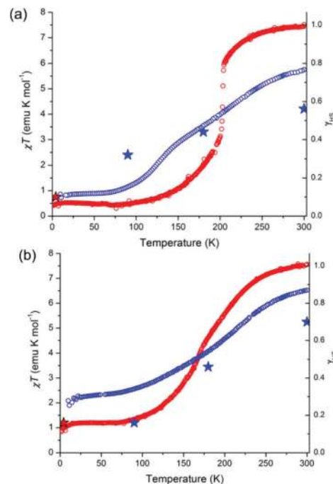
Fig. 34 Plot of \chi T and the high spin fraction ( \gamma_{\text{HS}} ) vs. T for the two HS Fe(II) sites attributed to being in \text{N}_6 coordination environments: red curves, as synthesized (wet) samples; blue curves, powder samples (a) [\text{Fe}_4(\text{L35})(\mu\text{-CN})_4](\text{BF}_4)_4 and (b) [\text{Fe}_4(\text{L35})(\mu\text{-CN})_4](\text{ClO}_4)_4 . Figures adapted with permission from ref. 124. Copyright 2014 ACS.
