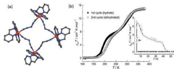
Fig. 35 (a) Crystal structure of the cation of [\text{Fe}_4(\text{L35})(\text{dca})_2](\text{BF}_4)_4 \cdot 2\text{H}_2\text{O} (b) plots of \chi_m T vs. T for [\text{Fe}_4(\text{L35})(\text{dca})_2](\text{BF}_4)_4 in two successive temperature cycles 300–100–380 K (square), and 380–100–380 K (circle). Inset: LIESST studies. Structure redrawn from CCDC data. (b) Reproduced with permission from ref. 126. Copyright 2011 John Wiley and Sons.
