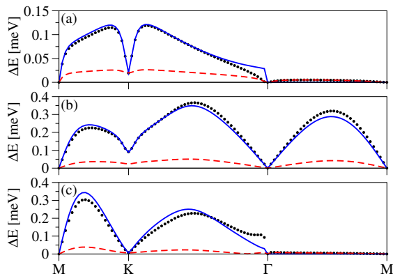
FIG. 7. (Color online) Spin-orbit splittings along the M-K- \Gamma -M line for the conduction (a), midgap (b), and valence bands (c); refer also to Fig. 6. First-principles data (dotted) are excellently reproduced by the phenomenological tight-binding model (solid) given by the Hamiltonian \mathcal{H}_0 + \mathcal{H}' + \mathcal{H}_{\text{SO}} from the text. The following orbital and SOC parameters were used in the tight-binding model as the best fits: T = 5.5 eV, \varepsilon_f = -2.2 eV, \Lambda_{\text{I}}^{\text{B}} = 3.3 meV, \Lambda_{\text{PIA}}^{\text{B}} = 7.3 meV, and \Lambda_{\text{R}} = 11.2 meV. Turning off the intra-atomic SOC of the fluorine adatom in the first-principles calculations reduces the spin-orbit splitting significantly (dashed line). This residual spin-orbit splitting can be attributed to the structural local sp^3 distortion caused by fluorination.
