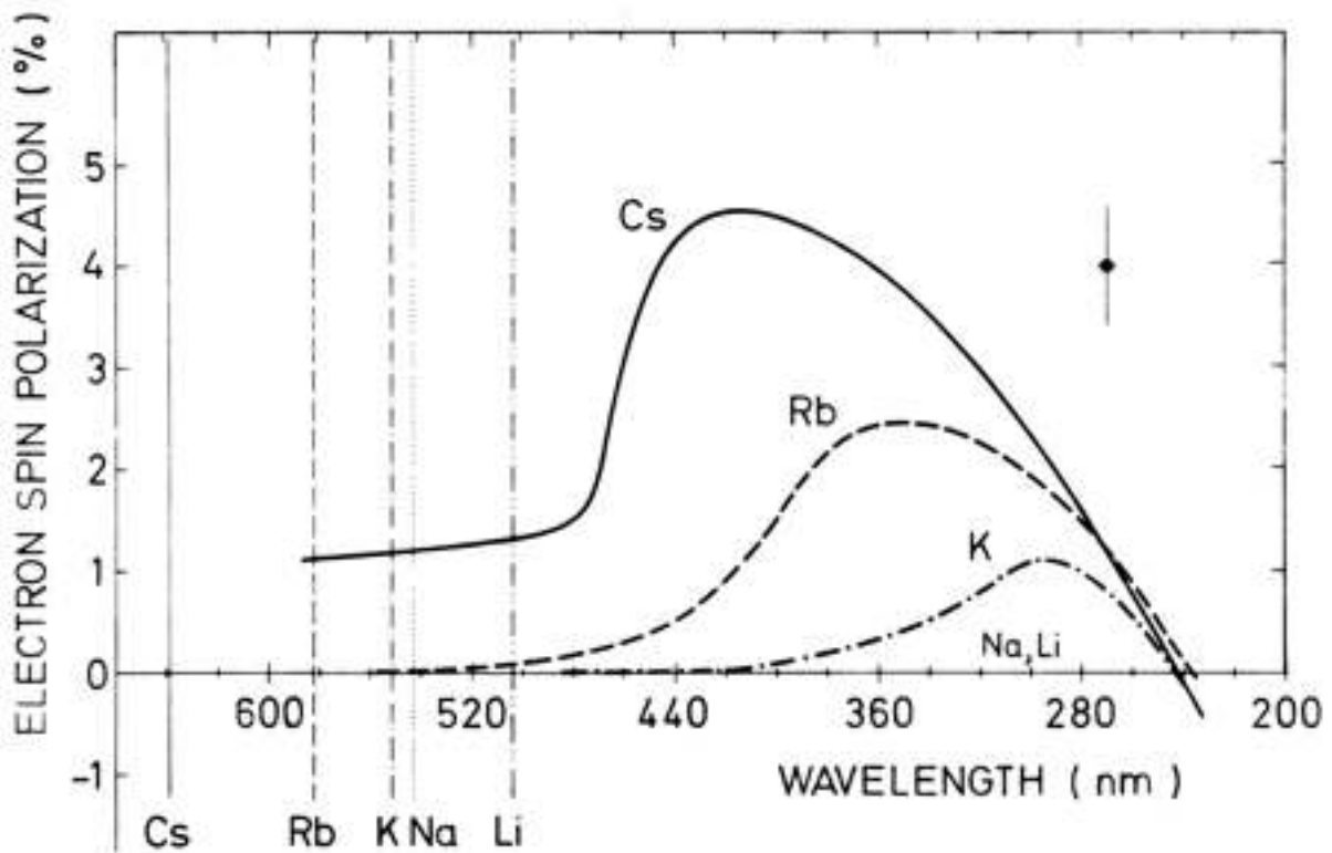
Fig. 3 Comparison of the emission angle integrated photoelectron spin polarization ejected by circularly polarized light from different solid alkali films. The curves denote the averaged experimental results. Their statistical uncertainties are described by the size of the single error bar shown outside the curves [15, 16].
