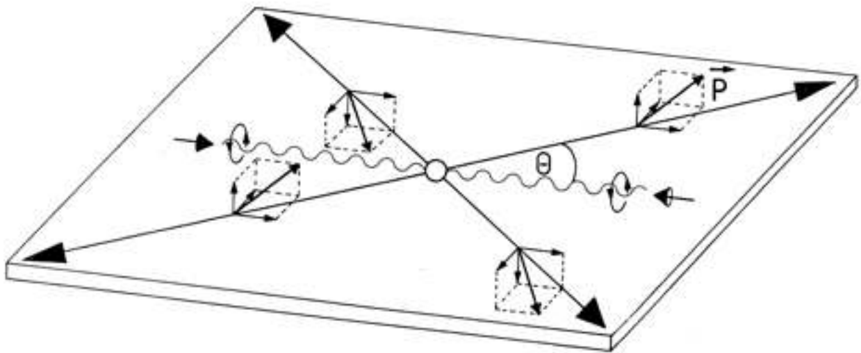
Fig. 12 Photoionization reaction plane using circularly polarized radiation with the three components of the spin polarization vector.
