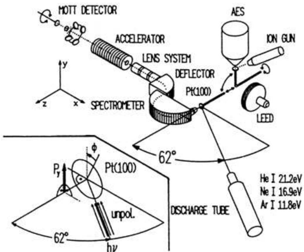
Fig. 20 Experimental set up [48, 49, 50].
