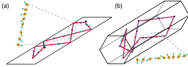
FIG. 1. (Color online) Quantum interference along time-reversed paths in (a) 2D and (b) 3D nanowires. In both cases an inversion symmetry induces spin precession in between (boundary) scattering events.
