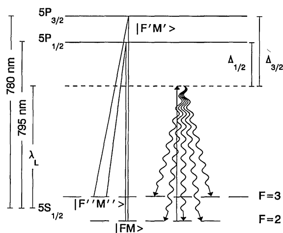
Fig. 1. Energy levels of ^{85}\text{Rb} showing spontaneous transitions from a linearly polarized laser. The ground-state hyperfine splitting is 3 GHz, and the excited-state hyperfine splitting, not shown, is of the order of 0.3 GHz. The laser wavelength \lambda_L is always to the red of both D lines, between 798 and 860 nm. For laser detunings greater than the excited-state fine- or hyperfine-structure splitting the scattering process can follow more than one path, as indicated by the solid lines.
