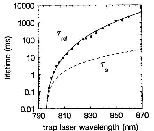
Fig. 2. Hyperfine population relaxation time as a function of trap laser wavelength. Experimental measurements are shown as filled circles. Calculated relaxation times are shown by the solid curve. The calculated mean time between spontaneous photon scattering events is shown by the dashed curve.
