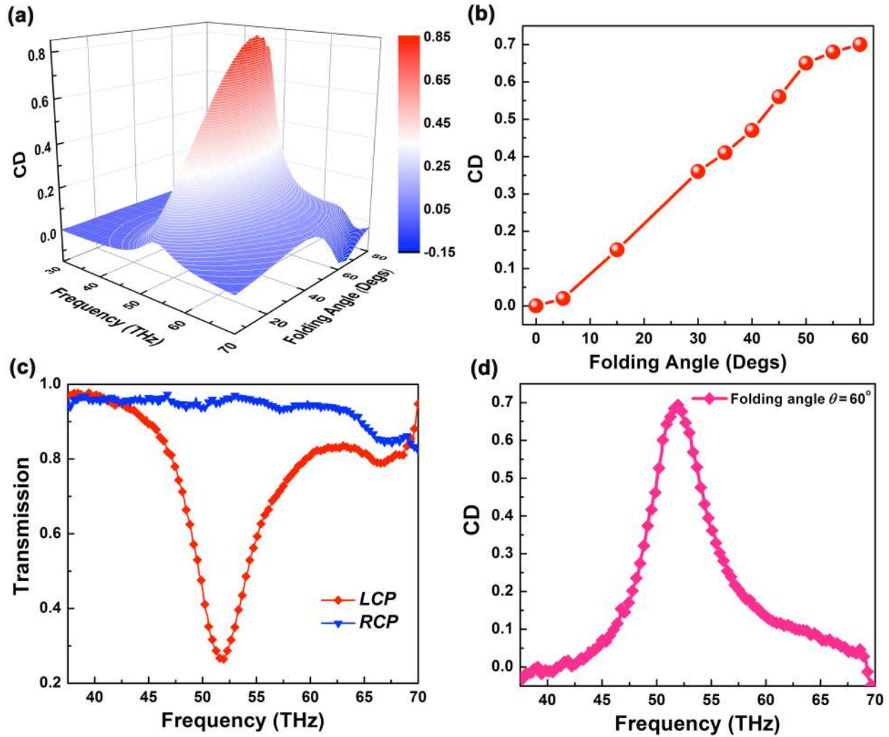
Figure 4. (a) The simulated CD spectra of the folded metasurface for a sweep of the folding angle from 5^\circ to 80^\circ . (b) Experimentally measured CD values at the chiral resonance frequency as a function of the folding angle. (c) Experimentally measured transmission spectra of the folded metasurface with folding angle \theta = 60^\circ under the illumination of LCP and RCP light. (d) CD curve of the folded metasurface with folding angle \theta = 60^\circ .
