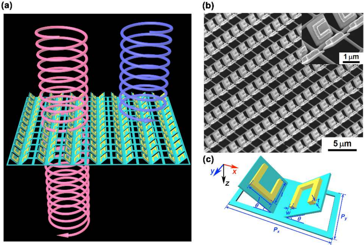
Figure 1. Design of folded metasurface which exhibits spin-resolved optical transmission. (a) Schematic diagram of optical dichroism from the 3D folded metasurface and the illumination configuration. (b) Scanning electron microscope image of the fabricated 3D folded metasurface. Inset: Zoomed in scanning electron microscopy image showing the well-defined structures. (c) A magnified schematic illustrates the composite of a 3D folding metasurface unit-cell with labeled dimensions. The parameters are: P_x = 4 \mu\text{m} , P_y = 2 \mu\text{m} , l = 900 \text{ nm} , w = 200 \text{ nm} , \theta = 50^\circ , t = 200 \text{ nm} . The thickness of the \text{SiN}_x film is 100 \text{ nm} .
