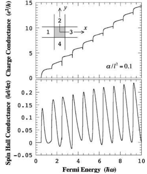
FIG. 1. Longitudinal charge conductance G_C and spin Hall conductance G_{\text{SH}} calculated as a function of Fermi energy E . In the calculation, the system size, and the SO coupling strength were set at W=60a and \alpha/l^2=0.1 , respectively. Inset is a schematic view of the four-terminal junction of QWs.
