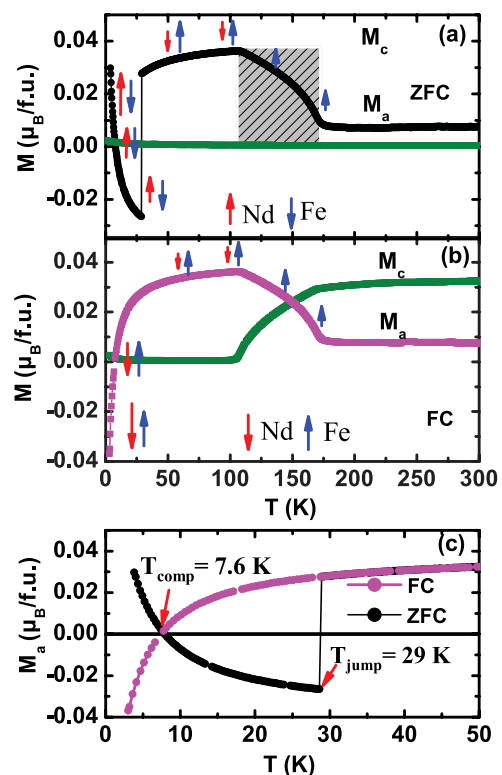
FIG. 1. (Color online) Temperature dependence of the magnetization M(T) of NdFeO 3 single crystal along a and c axes measured in (a) ZFC and (b) FC processes; (c) the magnified view of the ZFC and FC M(T) curves at low temperatures. The cooling and measuring fields are 100 Oe. The arrows in (a) and (b) represent the evolution of the effective magnetic moment of Fe (in blue) and Nd (in red) ions. The shadow in (a) marks the spin reorientation region of the Fe sublattice; the inset in (a) shows the image of the as-grown single crystal NdFeO 3 .
