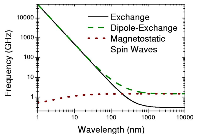
FIG. 1. (Color online) The frequency of exchange, dipole-exchange, and magnetostatic spin waves are plotted as a function of their wavelength for a 5-nm-thick film of YIG, neglecting anisotropy and assuming that the wave vector is parallel to the static magnetization.
