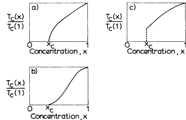
FIG. 12. Some simple possible behaviors for T_c(x) . In (a) and (b) we show a second-order "transition" with T_c(x) having either infinite slope [as in (a)] or finite slope [as in (b)] as x \rightarrow x_c . In (c) we show a first-order "transition." Elliott's arguments (Ref. 36) indicate that T_c(x) for the Ising model resembles diagram (a).
