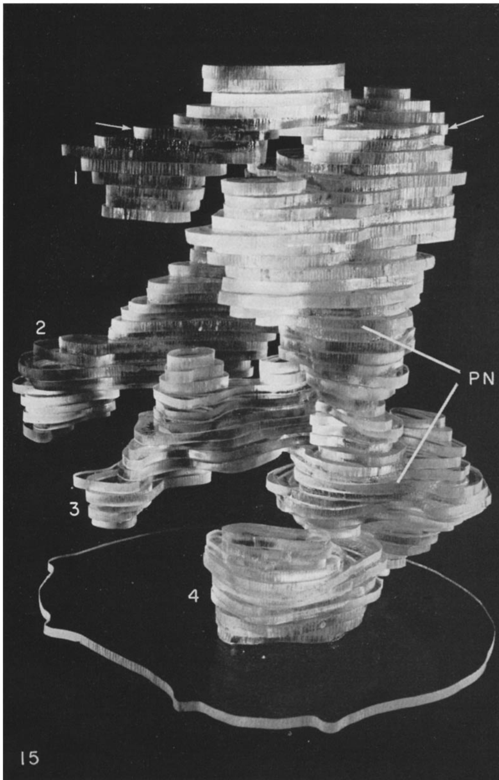
FIGURE 15 Sporulating yeast: meiosis II. A model based on a \text{KMnO}_4 -fixed cell (Fig. 13) made by tracing the nuclear envelope of each consecutive electron micrograph is shown. There is a large parent nucleus (PN), and four developing ascospore nuclei (Nos. 1-4) are budding from it. The arrows mark the position of the section shown in Fig. 14. The base plate shows the outline of the yeast ascus with two bud scars.
