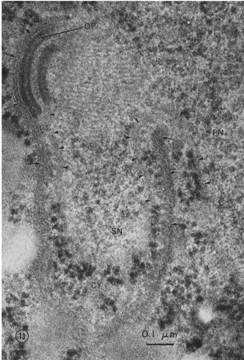
FIGURE 13 Sporulating yeast: meiosis II. Higher magnification of the early ascospore development is shown. The dark-staining structure is the spindle plaque which, at this stage, is at its maximum size and, which has a large outer plaque ( OP ) and a smaller inner plaque. Immediately adjacent to the outer plaque at the cytoplasmic side, is the prospore wall marked by arrows. The prospore wall has the shape of a shoe, which encloses nuclear material ( SN ) and cytoplasm ( CY ) somewhat like a foot surrounded by a sock. The prospore wall does not actually end on the nuclear envelope, which is marked with arrowheads. Thus, the cytoplasm of the ascus is continuous with the cytoplasm of the ascospore. The inner plaque appears to lie at the level of the nuclear membranes. The ascospore nucleus ( SN ) is continuous with the parent nucleus ( PN ), but the latter has no wall around it. \times 145,000 .
