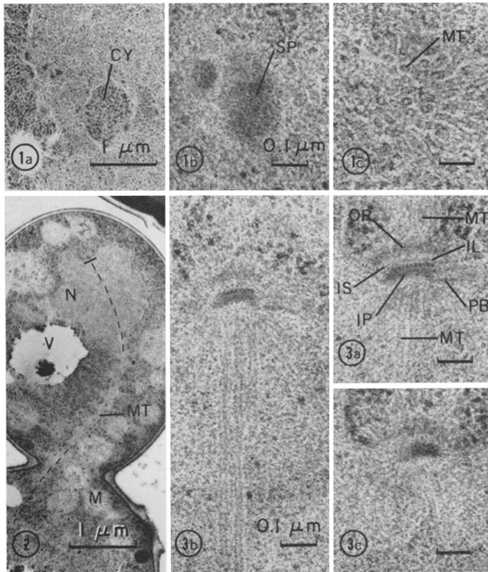
FIGURE 1 Budding yeast: serial sections of a spindle plaque cut perpendicular to the long axis of the spindle. In Fig. 1 a : underlying the plaque is a cytoplasmic invagination ( CY ) into the nucleus. \times 17,000 . Fig. 1 b : the spindle plaque ( SP ) is a disc-shaped structure, consisting of finely granular electron-opaque material. \times 93,000 . Fig. 1 c : radiating up from the plaque are the microtubules ( MT ). The scale line is 0.1 \mu\text{m} . \times 93,000 .
