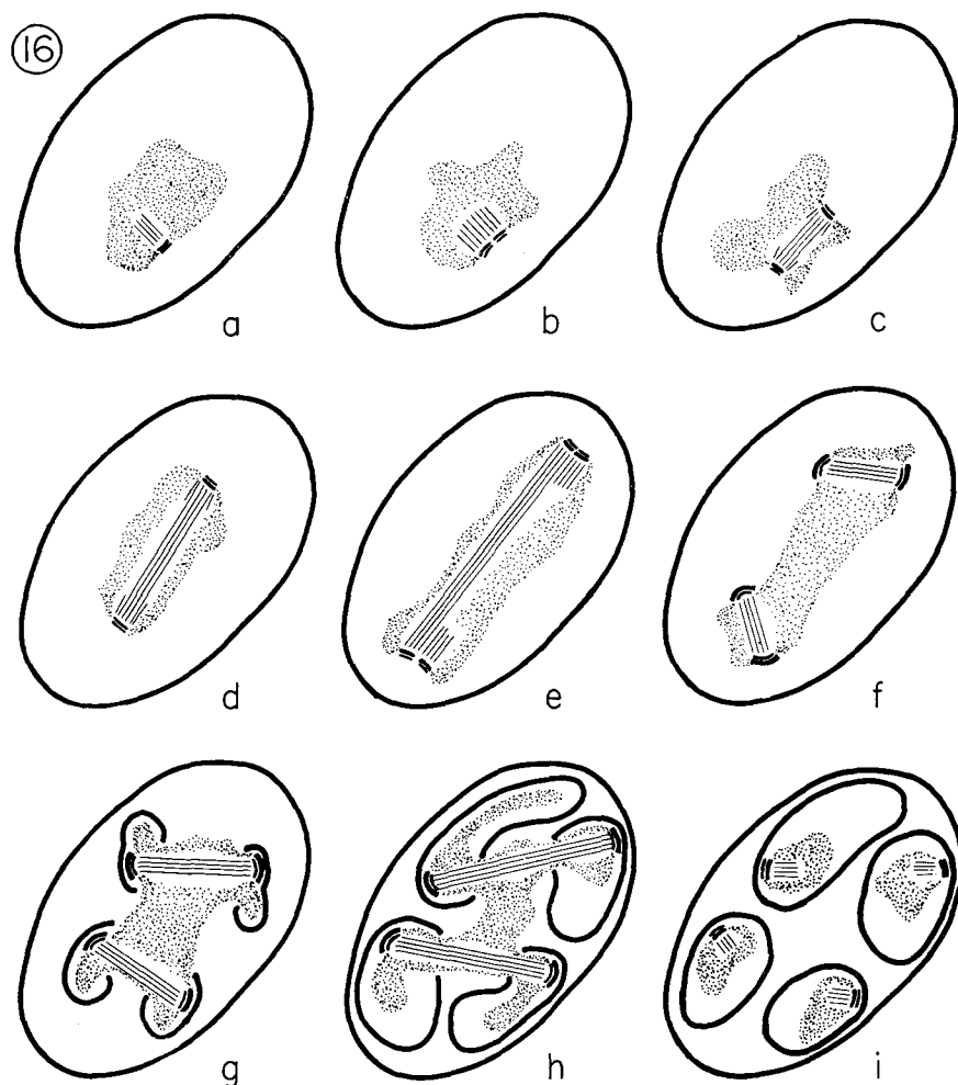
FIGURE 16 Sporulating yeast: summary. Figs. 16 a-16 i are sketches showing the development of spindles, spindle plaques, and ascospores.
