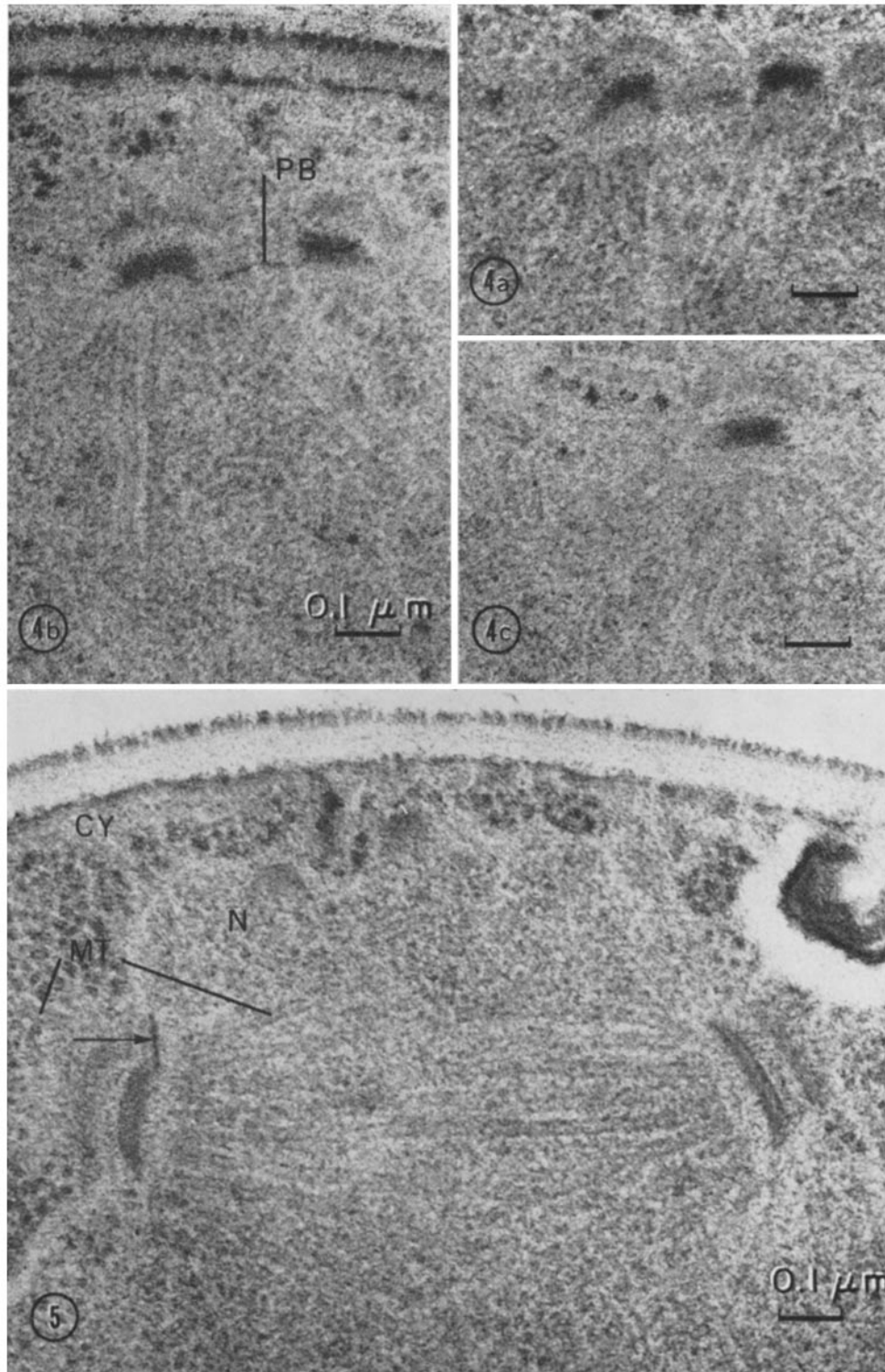
FIGURE 4 Budding yeast: serial sections of replicating plaques. In Figs. 4 a , 4 b , and 4 c , the two spindle plaques are connected by the plaque bridge ( PB ). Microtubules radiate from both plaques; some tubules intersect. The scale lines are 0.1 \mu\text{m} . \times 93,000 .
