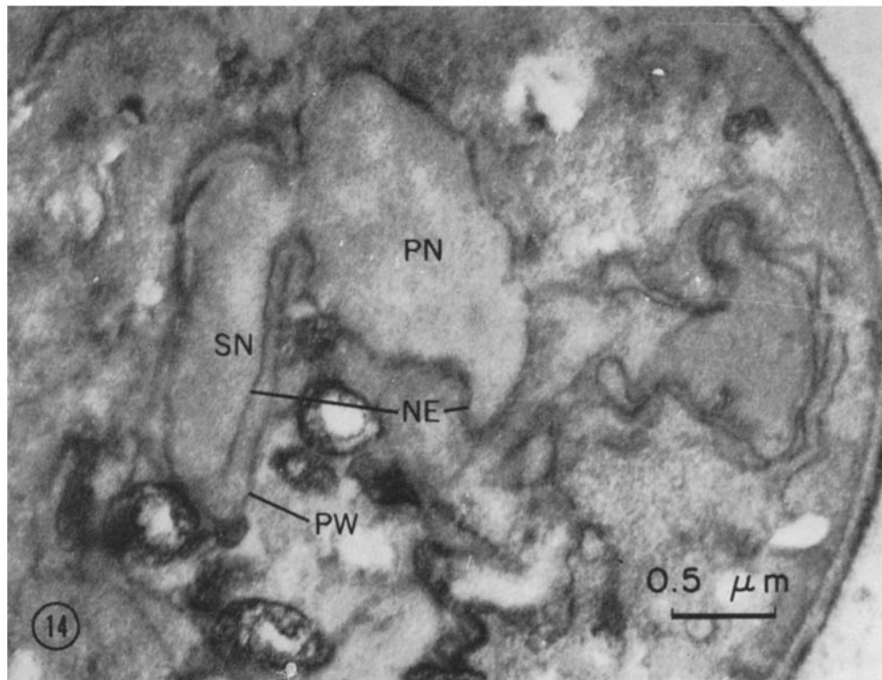
FIGURE 14 Sporulating yeast: meiosis II. A section of a \text{KMnO}_4 -fixed cell is shown, which should be compared with Fig. 13 for identification of parts. The complete nucleus is shown in the model of Fig. 15. The parent nucleus ( PN ) and spore nucleus ( SN ) are connected and they are surrounded by a single envelope ( NE ). The spore nucleus ( SN ) is surrounded by a second envelope, the prospore wall ( PW ), analogous in orientation to the prospore wall of Fig. 13. The parent nucleus ( PN ) has no second envelope. \times 30,000 .
