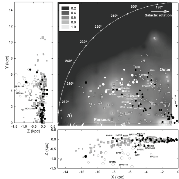
FIG. 3.—CO molecular cloud mass covering the mass ranges 0 < M_{\odot} \leq 0.5 (small gray squares), 0.5 < M_{\odot} \leq 1 (medium gray squares), and > 1 M_{\odot} (large gray squares), in units of 10^5 M_{\odot} smoothing onto the X - Y plane from May et al. (1988, 1997, 2007) data. For the smoothing process we use the nearest neighbors procedure and a 0.5 kpc kernel. The inset shows the mass scale of the smoothing in units of 10^5 M_{\odot} . A scale of Galactic longitudes and the Galactic rotation are also shown. Some clusters and BPs (filled and open circles, respectively) are indicated regarding their positions from the formal Galactic plane at b = 0^\circ . The bottom and left panels show the X - Z and Y - Z projections, respectively, of molecular clouds, clusters, and BPs. No CO smoothing was performed in these panels. The Sun is at (0, 0). Large symbols denote the new fields observed, listed in Table 1.
