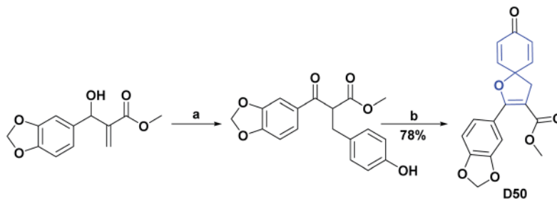
Scheme 47 Structures, reagents and conditions for the synthesis of spiro heterocycle [4.5.0] D50. (a) 4-Iodophenol, Et 3 N, Nájera's catalyst, 141 DMF, 110 °C, 3 h. (b) PIFA, anhydrous CH 3 CN, -10 °C, N 2 , 10–15 min.
