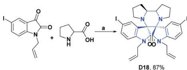
Scheme 26 Structures, reagents and conditions for the synthesis of spiro heterocycle [4.5.0] D18 . (a) toluene–MeOH, reflux, 2 h.
