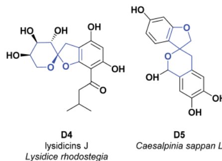
Fig. 5 Structures of spiro heterocycles [4.5.0] lysidicins J (D4) and D5.
