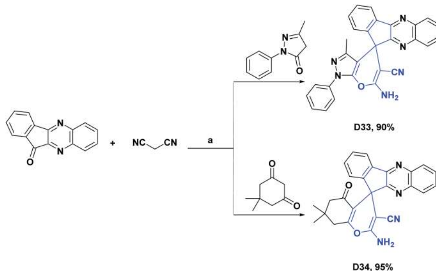
Scheme 37 Structures, reagents and conditions for the synthesis of spiro heterocycles [4.5.0] D33 and D34 . (a) APVPB, H 2 O, reflux, 5 h.
