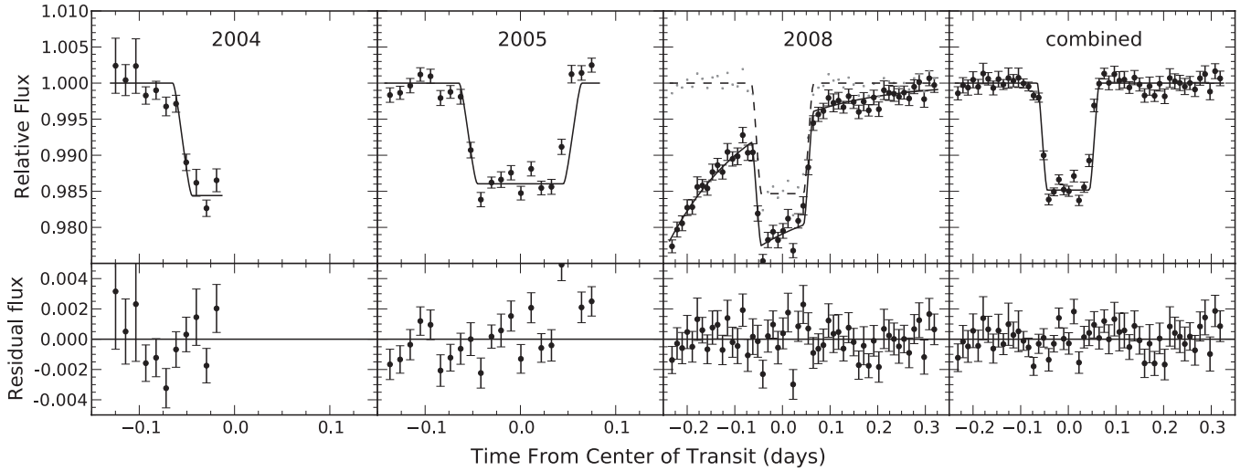
Figure 3. MIPS 24\ \mu\text{m} transits of HD 209458b. The top panels show photometry and the best-fit model, and the lower panels show the residuals to the fits. For plotting purposes, the data have been corrected for the MIPS 14-position sensitivity variations, normalized by the stellar flux, and binned by 70 points (for the individual transits) and by 210 points (for the combined data set). We also corrected for the ramp in the 2008 data set (corrected, binned data shown as small points) before combining the data to plot the data in the rightmost panel.
