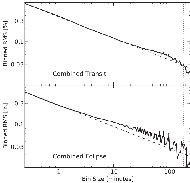
Figure 4. Dispersion of the binned residuals (solid lines) to the combined transit and eclipse light curve fits shown in Figures 3 and 7. On longer timescales, both fits exhibit a binned dispersion 10%–30% higher than expected from uncorrelated noise (dashed line). The dashed lines show the expectation for uncorrelated errors, which scale as N^{-1/2} . The vertical dotted line indicates the transit duration.
