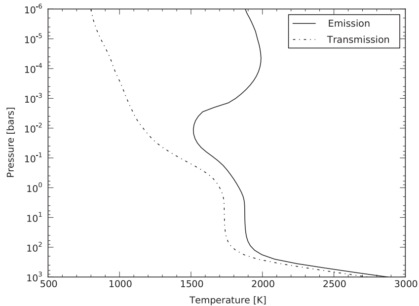
Figure 9. Temperature–pressure ( T – P ) profiles used to generate our model spectra. The dot-dashed curve is a planet-wide average T – P profile taken from a full ( 4\pi ) redistribution model, and is used to model the transmission spectrum shown in Figure 6. It includes TiO/VO opacity, but these species have only a minor effect since nearly all of the Ti/V has condensed out of the gas phase at these cooler temperatures. The solid curve is from a model assuming no redistribution of absorbed energy (making it hotter), and includes TiO/VO to drive the temperature inversion seen in Figure 8.
