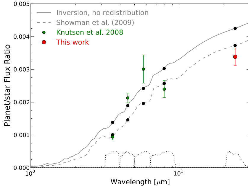
Figure 8. Measurements of the secondary eclipse depth of HD 209458b: previous Spitzer /IRAC photometry (Knutson et al. 2008) and our 24 \mu\text{m} measurement. The solid line is from a model assuming zero redistribution of incident flux and including gaseous TiO and VO to drive a temperature inversion; we show this model’s temperature–pressure profile in Figure 9. The dashed line is the emission spectrum from Showman et al. (2009). The solid black points without error bars represent the weighted averages of the models over the corresponding bandpasses (indicated at bottom).
