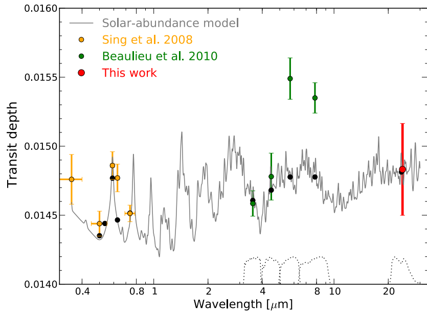
Figure 6. Measurements of the transit depth of HD 209458b: binned optical spectroscopy (Sing et al. 2008), previous mid-infrared photometry (Beaulieu et al. 2010), and our 24\ \mu\text{m} measurement. The solid line is a model generated using the (dot-dashed) temperature–pressure profile shown in Figure 9. The solid black points without error bars represent the weighted averages of the model over the corresponding bandpasses (indicated at bottom).
