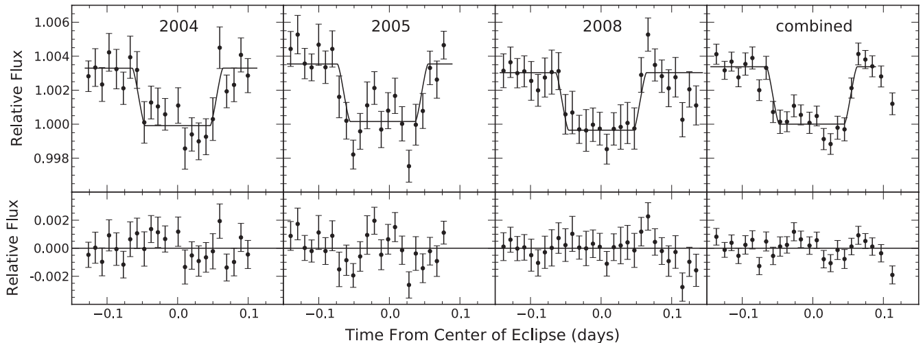
Figure 7. MIPS 24\ \mu\text{m} eclipses of HD 209458b. The top panels show photometry and the best-fit models, and the lower panels show the residuals to the fits. For plotting purposes the data have been corrected for the MIPS 14-position sensitivity variations, normalized by the stellar flux, and binned by 70 points (for the individual eclipses) and by 210 points (for the combined data set).
