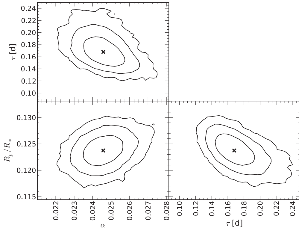
Figure 5. Posterior distributions of the ramp parameters ( \alpha , \tau ) and R_p/R_* , estimated from the MCMC analysis of the 2008 transit data. The “x” symbols indicate the best-fit parameters listed in Table 3, and the lines indicate the 68.27%, 95.45%, and 99.73% confidence intervals. The elements of these parameters’ covariance matrix are listed in Table 4.
