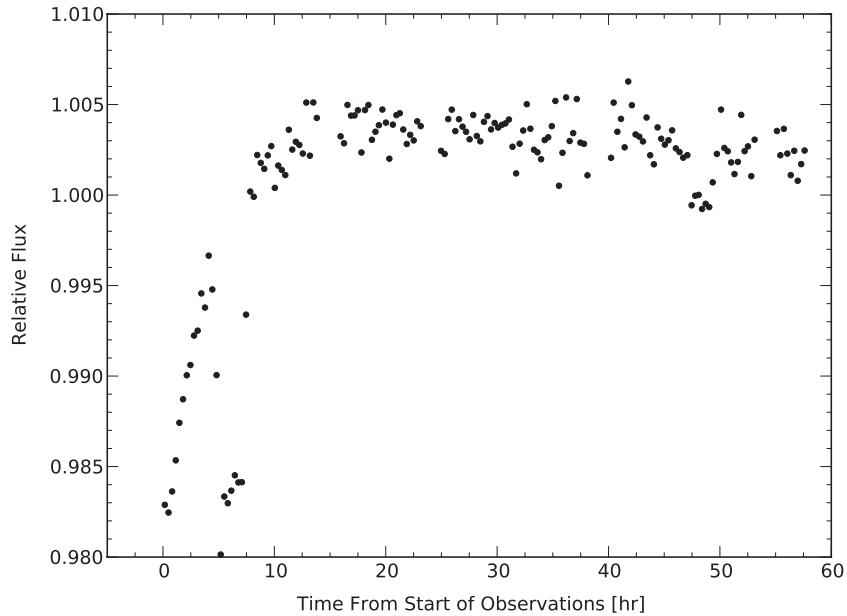
Figure 1. MIPS 24\ \mu\text{m} photometry of the HD 209458 system, showing the detector ramp (0–10 hr), transit (5 hr), and eclipse (48 hr). For plotting purposes, the data have been binned to lower temporal resolution. A slight ( \sim 0.2\% ) flux decrease is apparent from 10 to 58 hr. This could be influenced by planetary phase variations, but the similarity to the purely instrumental effects seen in Figure 2 precludes an unambiguous distinction between the two effects.
