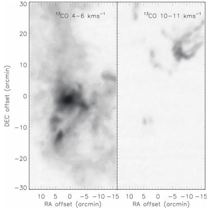
Fig. 6. ^{13}\text{CO} intensity maps, integrated for two velocity intervals, of the molecular cloud associated with NGC 2264 cluster (see Ridge et al. 2003). The bulk of the molecular cloud has V_{\text{LSR}} between 4 \text{ km s}^{-1} and 6 \text{ km s}^{-1} , and a clear separate component is present at 10\text{--}11 \text{ km s}^{-1} corresponding to the Fox Fur Nebula (compare with Fig. 5). The contours are the same for both panels, starting at 1.5 \text{ K km s}^{-1} with increments of 1.5 \text{ K km s}^{-1} .
