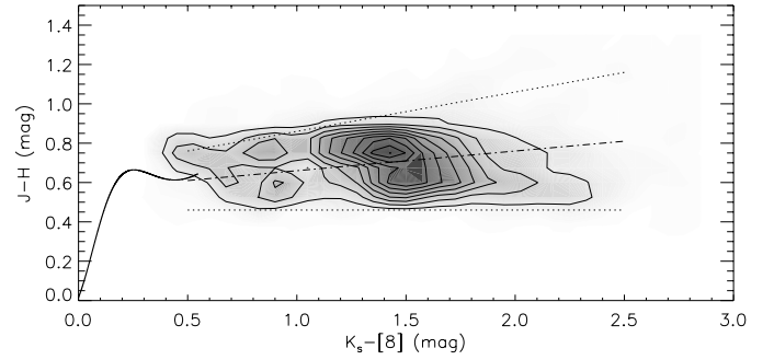
Fig. A.3. Synthetic color-color diagram built using the models shown in Figs. A.1 and A.2 with an IMF sampling (Kroupa 2001; Robitaille et al. 2006). The solid line represents the main sequence, the dot-dashed line the empirical disk locus, and the dotted lines the 5\text{-}\sigma error loci discussed in Sect. 3.3, and shown in Fig. 8 and Table 3.
