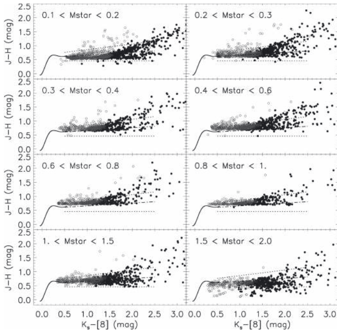
Fig. A.2. Same as Fig. A.1, except for models of disks with inclination angles greater than 75^\circ .
