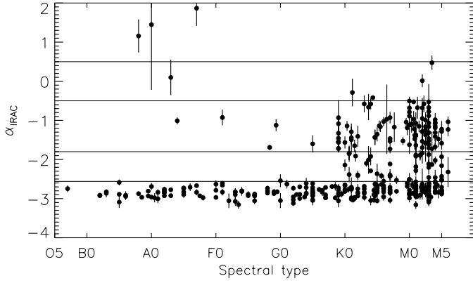
Fig. 3. Variation in \alpha_{\text{IRAC}} with spectral type. The horizontal thick lines correspond to the limits used to classify the evolutionary phases of protostars and PMS objects.
