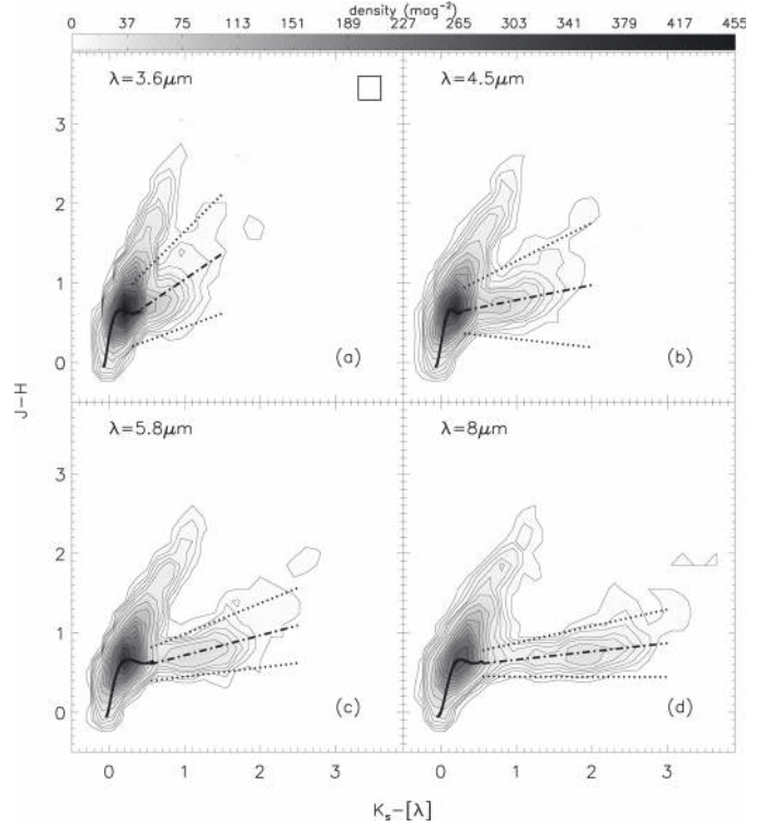
Fig. 8. NIR+IRAC colour–colour Nyquist-sampled density diagrams for sources in the IRAC sample. The beam size is 0.3 \times 0.3 mag and is represented by a pixel in the upper right corner of panel a ). The contours are the same for each diagram and correspond to 3, 6.5, 10, 15, 20, 30, 50, 75, 100, 125, 150, 175, 200, 250, 300, and 400 sources \text{mag}^{-2} . The solid black curve corresponds to the main sequence of the Pleiades (see Lada et al. 2006). The dashed-dotted lines correspond to the loci of diskless sources for each colour–colour space (see Table 3). The dotted lines correspond to 3\text{-}\sigma ( 5\text{-}\sigma ) error in the disk loci for the upper (lower) two panels.
