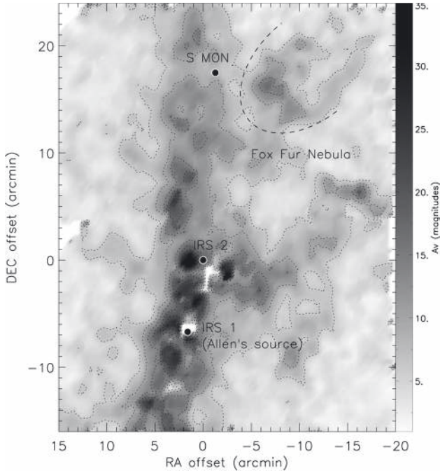
Fig. 5. FLAMINGOS dust extinction map of the molecular cloud associated with the NGC 2264 cluster. The map is centred on (\alpha, \delta)(J2000.0) = (6^{\text{h}}41^{\text{m}}02.6^{\text{s}}, +09^{\circ}36'12.2'') . The spatial resolution is 50'' and the contours range from 6 to 30 mag in steps of 4 mag. For positional reference, the sources IRS 1, IRS 2, and S Mon are represented by filled circles, while the approximate southeastern edge of the Fox Fur Nebula is marked by a dashed curve.
