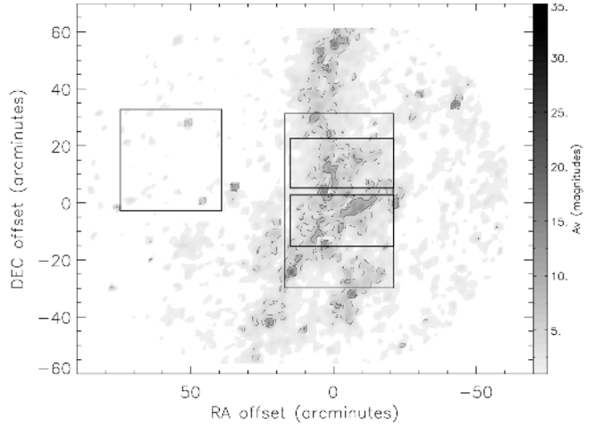
Fig. 4. Nyquist sampled, 2.5' resolution 2MASS dust extinction map of the molecular cloud associated with NGC 2264. The map is centred on (\alpha, \delta)(\text{J2000.0}) = (6^{\text{h}}41^{\text{m}}02.6^{\text{s}}, +09^{\circ}36'12.2'') . The dashed contour corresponds to A_V = 4 mag, while the solid contour corresponds to A_V = 8 mag. The box on the eastern part of the map indicates the size and location of the control field, while the larger box centred on the molecular cloud represents the area surveyed by IRAC. The FLAMINGOS fields, also centred on the cloud, are represented by boxes drawn with thicker lines.
