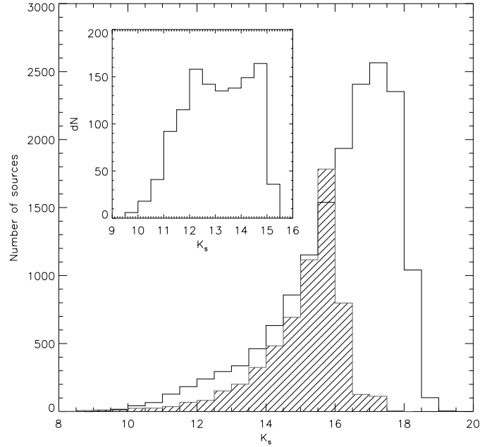
Fig. 11. Comparison of the NGC 2264 FLAMINGOS K_s -band luminosity function (KLF) (solid black line) to the reddened 2MASS control field KLF (red hatched-line histogram). The histogram in the inset shows the differential KLF, with 1194 sources.
