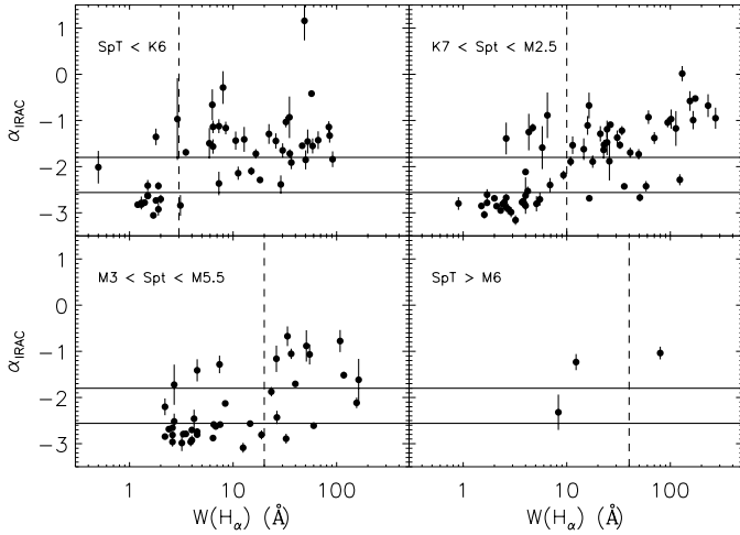
Fig. 10. Comparison of the H\alpha equivalent width ( WH\alpha ) with \alpha_{\text{IRAC}} for sources of different spectral type (SpT). The horizontal lines mark the separation between disk-less sources, sources with anaemic, and sources with thick disks (see Table 2), while the vertical dashed lines separate accreting and non-accreting sources.
