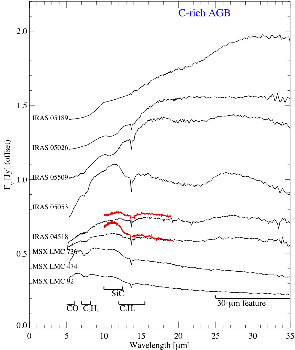
Figure 2. Spectra of C-rich AGB stars observed in the LMC. The molecular ( \text{C}_2\text{H}_2 and CO) and dust (SiC and 30 \mu\text{m} ) features are indicated. Fluxes are offset by arbitrary amounts for clarity. High-resolution spectra of IRAS 04518–6852 and MSX LMC 736 are plotted in red lines. The spectra are plotted in order of the underlying continuum temperature, from cooler (top) to warmer (bottom).
