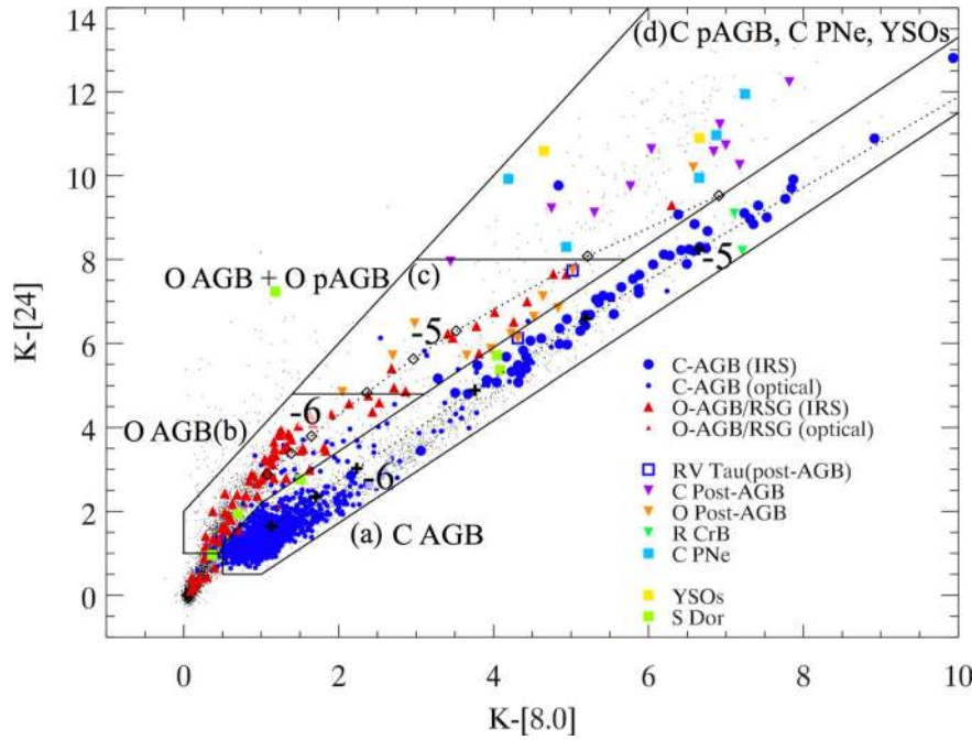
Figure 10. The K_s –[8.0] versus K_s –[24] colour–colour diagram of the LMC objects. The black dots show all of the data in the SAGE data base, combined with 2MASS photometric data. Other symbols show the sources with known spectral classifications. C-AGB: carbon-rich AGB stars, where ‘IRS’ represents objects classified from Spitzer IRS observations, and ‘optical’ represents objects classified on the basis of optical spectra. O-AGB: oxygen-rich AGB stars, RV Tau: RV Tauri stars, C post-AGB: carbon-rich post-AGB stars, O post-AGB: oxygen-rich post-AGB stars, R CrB: R CrB stars, C PNe: carbon-rich PNe. The boxes highlight the object types typically found in the colour ranges indicated. Carbon-rich post-AGB stars are found in region (d) and are well separated from carbon-rich AGB stars, but region (d) also contains PNe and YSOs. Oxygen-rich post-AGB stars are found in region (c). The two dotted lines show the typical colour at a given mass-loss rate of oxygen-rich (diamonds) and carbon-rich (plus signs) AGB stars. The diamond and plus sign symbols show the mass-loss rates 3 \times 10^{-7} , 6 \times 10^{-7} , 1 \times 10^{-6} , 3 \times 10^{-6} , 6 \times 10^{-6} , 1 \times 10^{-5} , 3 \times 10^{-5} and 6 \times 10^{-5} M_{\odot} \text{ yr}^{-1} , and the colours for 1 \times 10^{-6} and 1 \times 10^{-5} M_{\odot} \text{ yr}^{-1} are indicated with –6 and –5.
