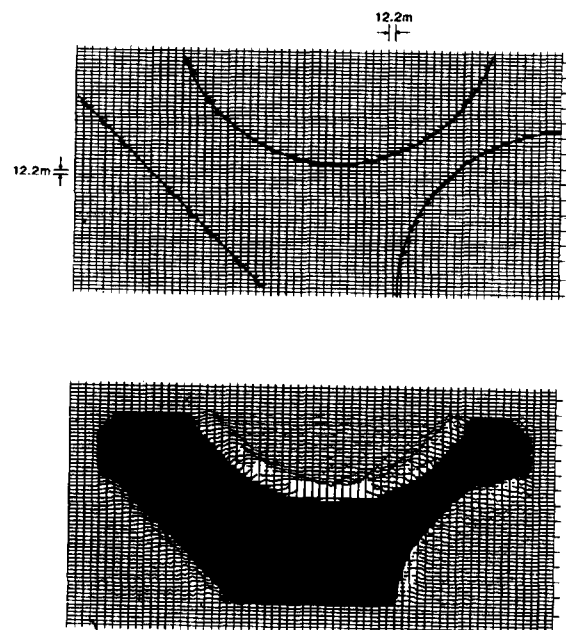
FIG. 9. (upper) Reflector locations for the French model obtained by taking first differences of the 3-D velocity field at a depth of 0.853 km. (lower) Corresponding depth slice after the split-step Fourier migration. The edges of each dome are correctly imaged. Figure 8 indicates the position of this depth slice in section format.
