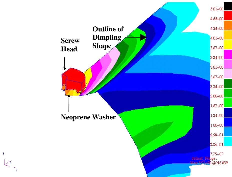
(b) Deformed Sheeting (deformation contours in mm)
