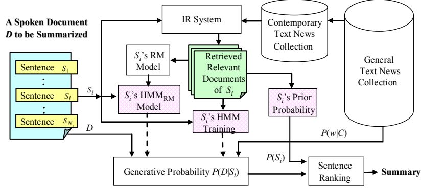
Figure 1: A schematic depiction of a probabilistic generative framework for extractive spoken document summarization using information from documents retrieved from a text collection.
