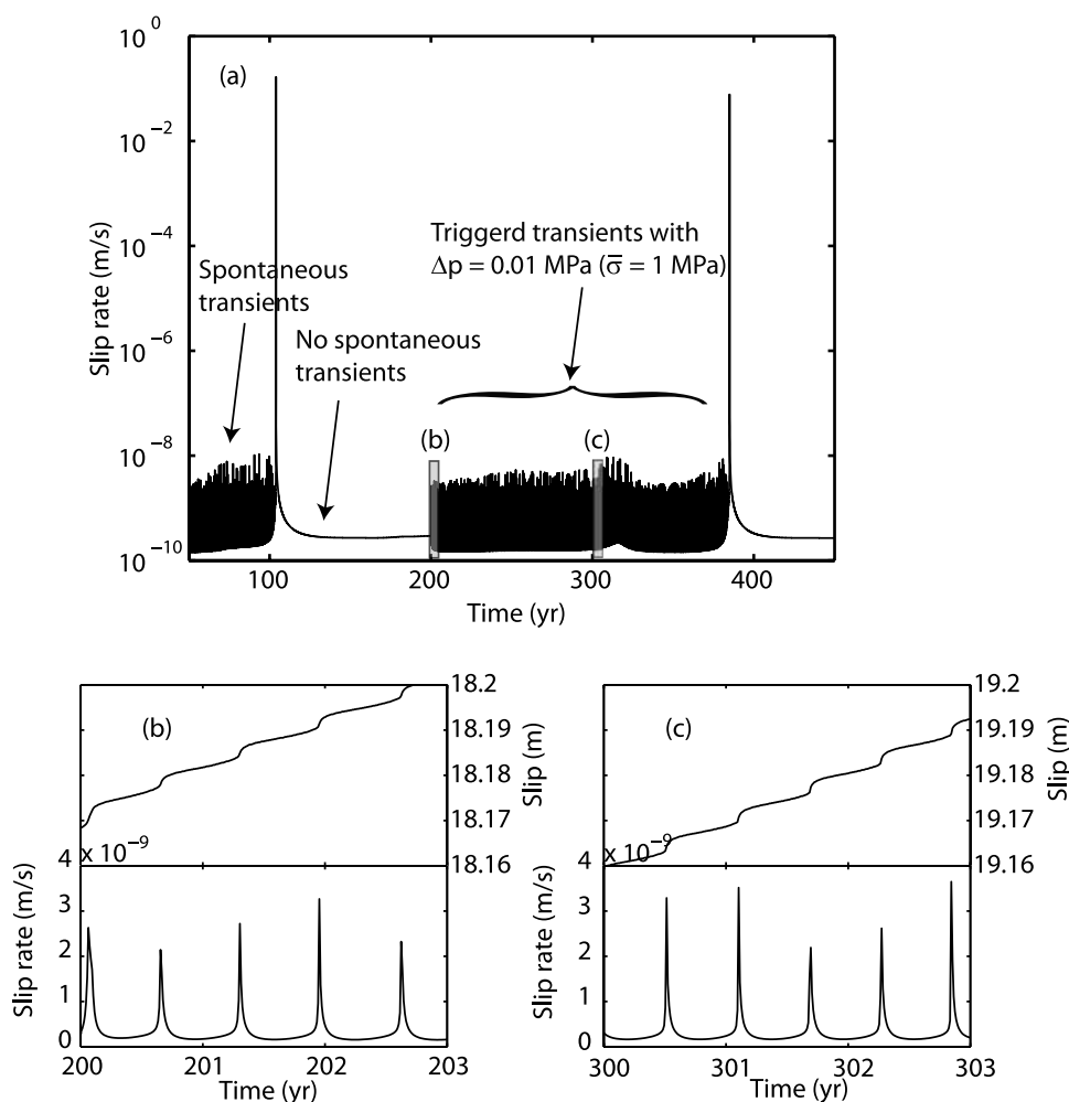
Figure 19. Unlocked seismogenic zone model: \bar{\sigma} = 50 MPa updip until 62.5 km and 1 MPa downdip from 70.2 km, with exponential decay between the two downdip locations. L correspondingly decreases from \sim 8 mm to 110 \mu\text{m} over the same range. Spontaneous transients are seen in the earthquake cycle before \sim 105 years but missing after. A one-time step perturbation of \delta p = 1\% \bar{\sigma} = 0.01 MPa is introduced at t = 200 years, from downdip 72 to 240 km. Quasiperiodic transients are triggered, until the next thrust earthquake.
