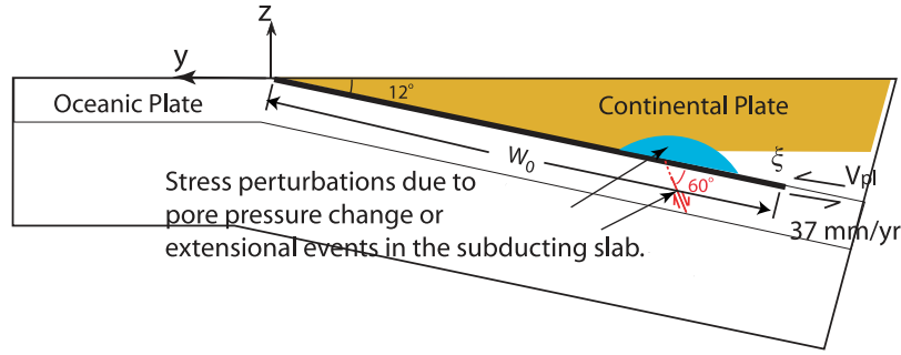
Figure 1. Two-dimensional subduction model. The parameter y is the horizontal direction opposite to the plate convergence, z is the vertical direction, and x (not shown) is the along-strike direction, perpendicular to the y - z plane. A rate- and state-dependent friction law is applied to fault 0 < \xi < W_0 . A uniform motion at plate convergence rate V_{pl} is imposed at W_0 < \xi < +\infty . Stresses resulted on the thrust fault due to an extensional event in the subducting slab or pore pressure changes from dehydration fluid release are considered possible sources of perturbation, as discussed in section 4.
