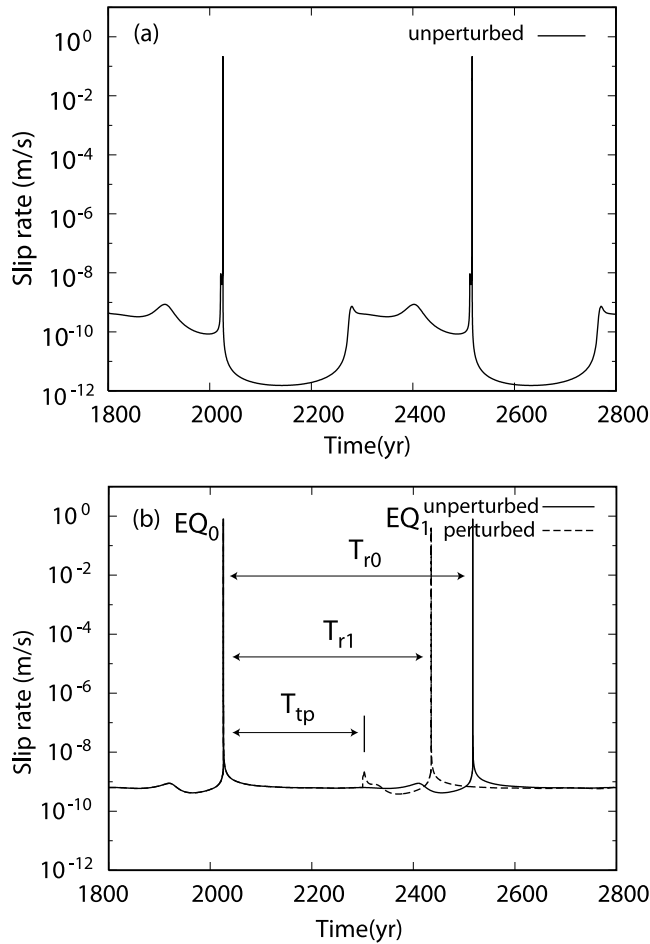
Figure 14. Slip rate (solid line without perturbation) at two representative downdip distances: (a) 48 km, in the nucleation zone, (b) 75 km, near the frictional stability transition. EQ_0 is the last thrust earthquake before perturbation, and EQ_1 is the first thrust earthquake after perturbation and triggered transients. T_{r0} is earthquake recurrence interval without perturbation; T_{r0} \approx 500 years here. T_{tp} is the interval between EQ_0 and the time when perturbation is introduced. T_{r1} is the interval between EQ_0 and EQ_1 .
