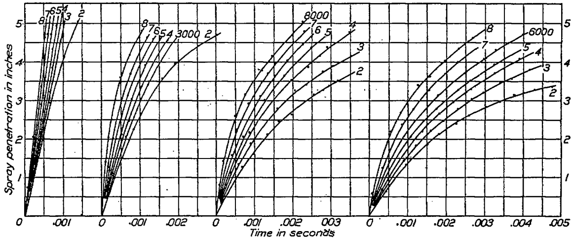
FIG. 9. Chamber pressure, atmospheric. Fuel pressure, 2,000 to 8,000 lb./sq. in. FIG. 10. Chamber pressure, 100 lb./sq. in. gage. Fuel pressure, 2,000 to 8,000 lb./sq. in. FIG. 11. Chamber pressure, 200 lb./sq. in. gage. Fuel pressure, 2,000 to 8,000 lb./sq. in. FIG. 12. Chamber pressure, 300 lb./sq. in. gage. Fuel pressure, 2,000 to 8,000 lb./sq. in. Effect of fuel pressure on penetration
