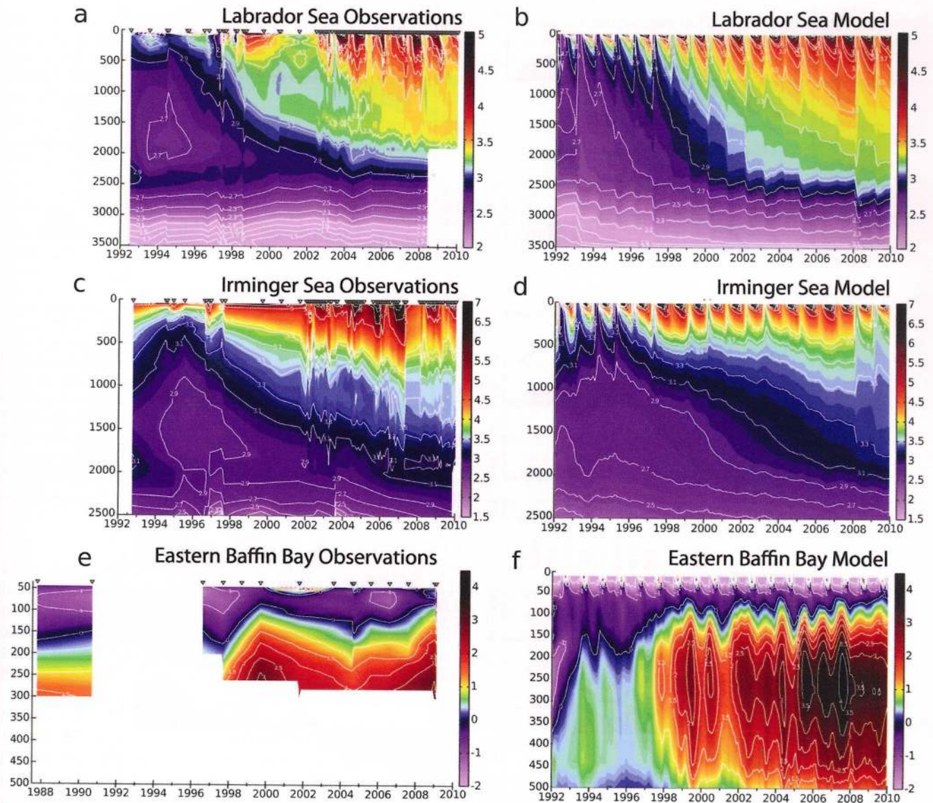
Fig. 2. Comparison of subsurface temperature along the AR7W line (see dotted black box in Fig. 1a) in the central Labrador Sea from (a) in situ data and (b) ECCO2 4 km Arctic Ocean solution for the time period 1992–2009 minus an absolute offset of 0.4^{\circ}\text{C} . Similar plots in (c) and (d) along the AR7E line in the Irminger Sea (Fig. 1a), and (e) and (f) for the Eastern Baffin Bay evaluation box (Fig. 1a). Triangles in (a), (c) and (e) denote the availability of observations. Temperature is linearly interpolated in between except in (e) between 1991 and 1996 where the data gap is too large.
