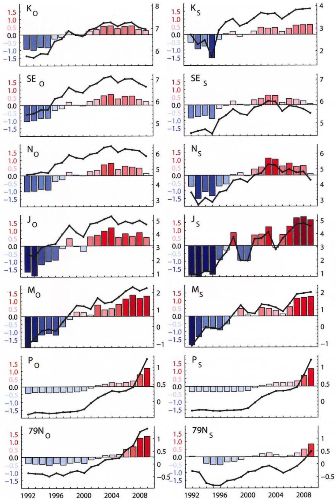
Fig. 3. Regional changes in subsurface ocean temperature from the 4 km ECCO2 simulation for the time period 1992–2009 minus an absolute offset of 0.4^{\circ}\text{C} . Left column is for off-shelf sites (triangles in Fig. 1a); right column is for on-shelf sites (diamonds in Fig. 1a). The size of the three-dimensional boxes used to calculate annual-mean subsurface temperatures is listed in Table 2. Left vertical axis indicates anomalies in subsurface temperature in reference to the average over the entire time period, between -1.5 and +1.5^{\circ}\text{C} , with vertical bars colored in red for positive anomalies and blue for negative anomalies. Right vertical axis in black is absolute subsurface temperature, with a scale that varies from site to site but not between on-shelf and off-shelf, except for K_O and K_S . Absolute temperature and anomaly calculations are insensitive to the particular trough or off-shelf location near each region ( \pm 0.2^{\circ}\text{C} ) but are somewhat sensitive to the depth range (shelf) and offshore extent (off shelf) over which the calculation is made. Hence, both on- and off-shelf averaging volumes use the same depth range, chosen to be below the seasonal mixed layer and above on-shelf waters without significant temporal variability. The off-shelf volumes span the IW component of the boundary current where possible, or comparably sized regions off the shelf where not ( P_S ).
