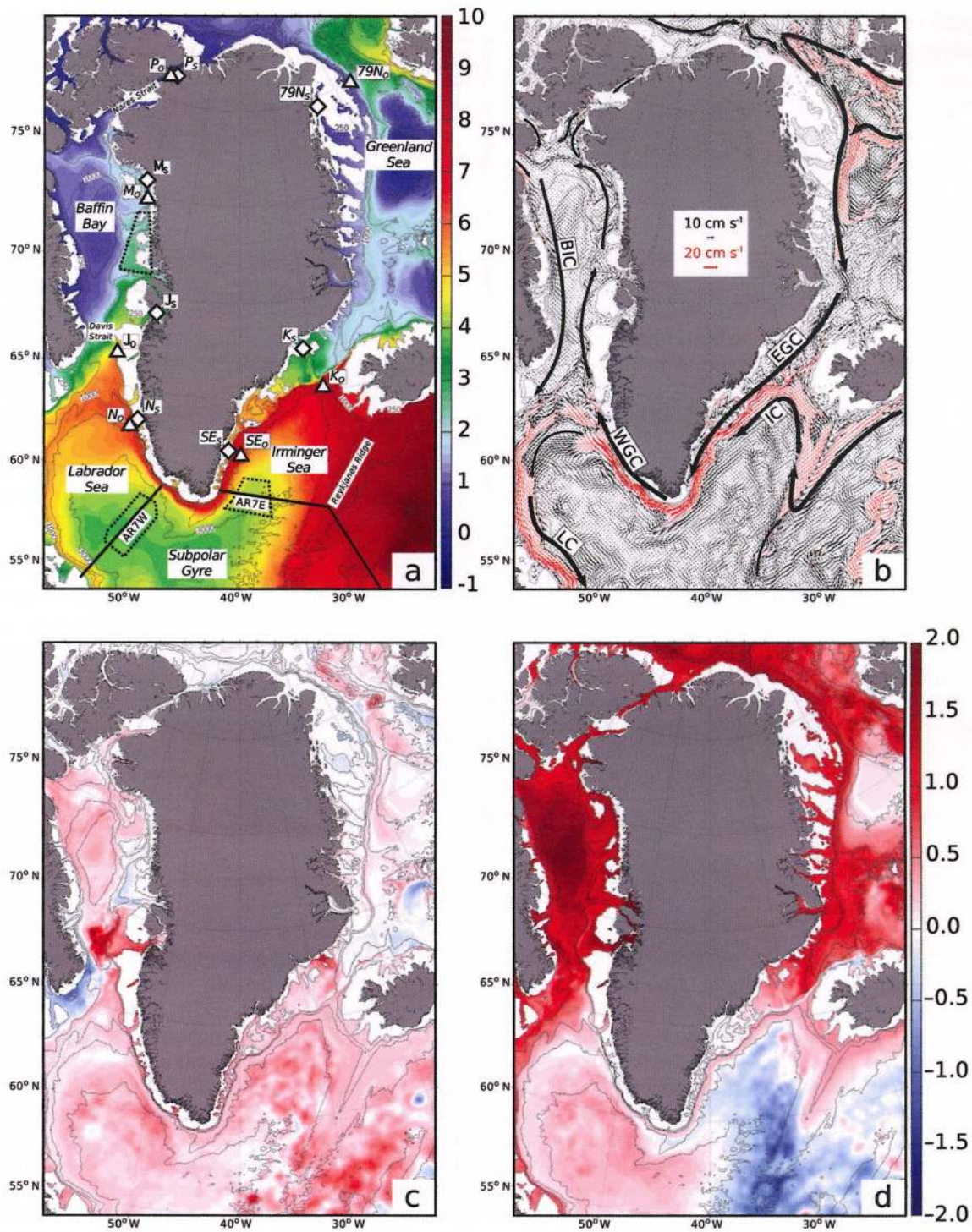
Fig. 1. Subsurface ocean temperature from the 4 km ECCO2 simulation overlain on IBCAO isobaths (Jakobsson and others, 2008). (a) Averaged for the time period 1992–2009 at 250 m depth (white areas are shallower than 250 m) with major locations discussed in the text. Sites are Kangerdlugssuaq Gletscher ( K_O and K_S ), southeast Greenland ( SE_O and SE_S ), Nuuk ( N_O and N_S ), Jakobshavn Isbræ ( J_O and J_S ), Melville Bay ( M_O and M_S ), Petermann Gletscher ( P_O and P_S ) and 79 North glacier ( 79N_O and 79N_S ). The AR7W, AR7E and eastern Baffin Bay evaluation boxes discussed in Figure 2 are dotted black lines. Diamonds (triangles) indicate the locations of on-shelf (off-shelf) three-dimensional boxes used to calculate the yearly-mean subsurface temperatures plotted in Figure 3. (b) Water velocity ( \text{cm s}^{-1} ) at 250 m depth with location of major ocean currents: Irminger Current (IC), East Greenland Current (EGC), Labrador Current (LC) and West Greenland Current (WGC). (c, d) The 2001 (c) and 2009 (d) mean temperature anomalies at 250 m from the model with respect to the 1992–2009 simulation period.
