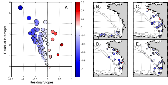
Figure 3. Size structure characteristics of residuals between NBSS estimated by the LOPC and by the WP2/Zs procedure. The color map indicates the value of the slope of the residuals (blue for negative slope, red for positive ones and white for null slopes). The size of points indicates the value of the intercept of residuals (the bigger the points, the larger the intercepts). (a) shows the relation between the slope and the intercept of residuals. (b–e) show the spatial distribution of residuals for the four cruises in which data are available for both LOPC and WP2/Zs (b: PELACUS 2007, c: PELGAS 2009, d: PELGAS 2010 and e: PELGAS 2011) using the same color map but size of points being divided by three for clarity.
