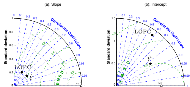
Figure 5. Taylor diagram (Taylor, 2001) of the correlation ( R ), the centered root mean square difference (RMSD) and standard deviation (STD) between NBSS parameters (a: slope and b: intercept) estimated by the WP2/Zs and estimated by the LOPC (black plain circles) and after the PLS (partial least square) regression performed on the LOPC ( \hat{Y} , black plain stars). The white square indicates the maximum ( R = 1 , RMSD = 0 and STD = 1).
