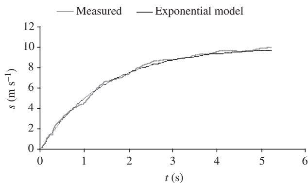
Fig. 2. Actual (gray, thick line) and modelled (black, thin line) forward speed s ( \text{m s}^{-1} ) as a function of time t (s) at the onset of a typical 100 m run for subject 7. Actual speed was accurately described by: s(t) = 10.0 * (1 - e^{-t/1.42}) . The maximal speed ( s_{\text{max}} ) was 10.0 \text{ m s}^{-1} .
