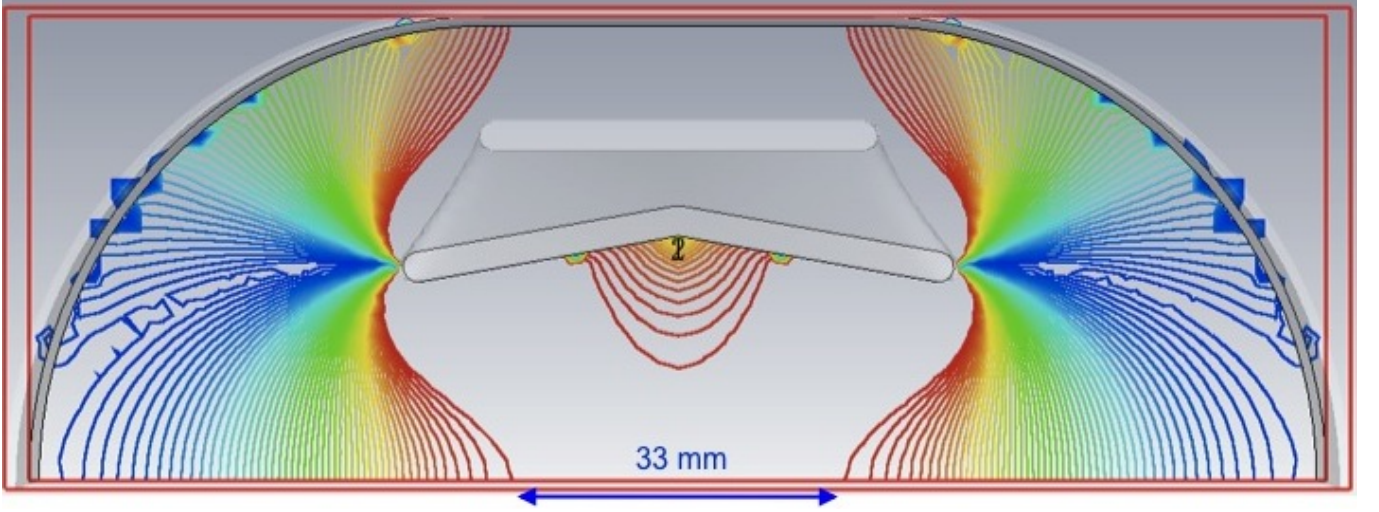
FIG. 18. Transverse electric field homogeneity. The isolines are spaced by 2% changes of the value of the deflecting field.
