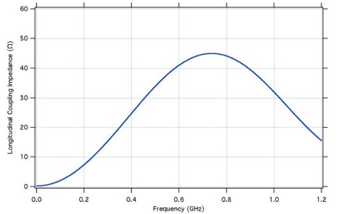
FIG. 19. Longitudinal beam coupling impedance for a 10 cm long stripline kicker module as evaluated by a virtual coaxial wire measurement.
