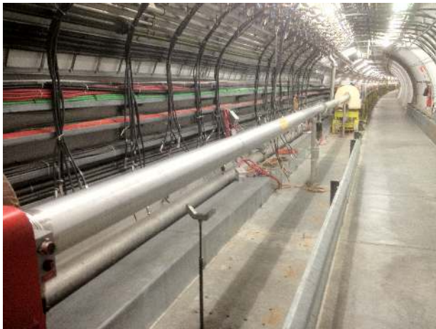
FIG. 2. Precise location in LSS3 of the SPS where the new kicker system will be installed. About 13 m of longitudinal space is available, but only about 8 m of that space is usable because of beam aperture (stay-clear) considerations.
