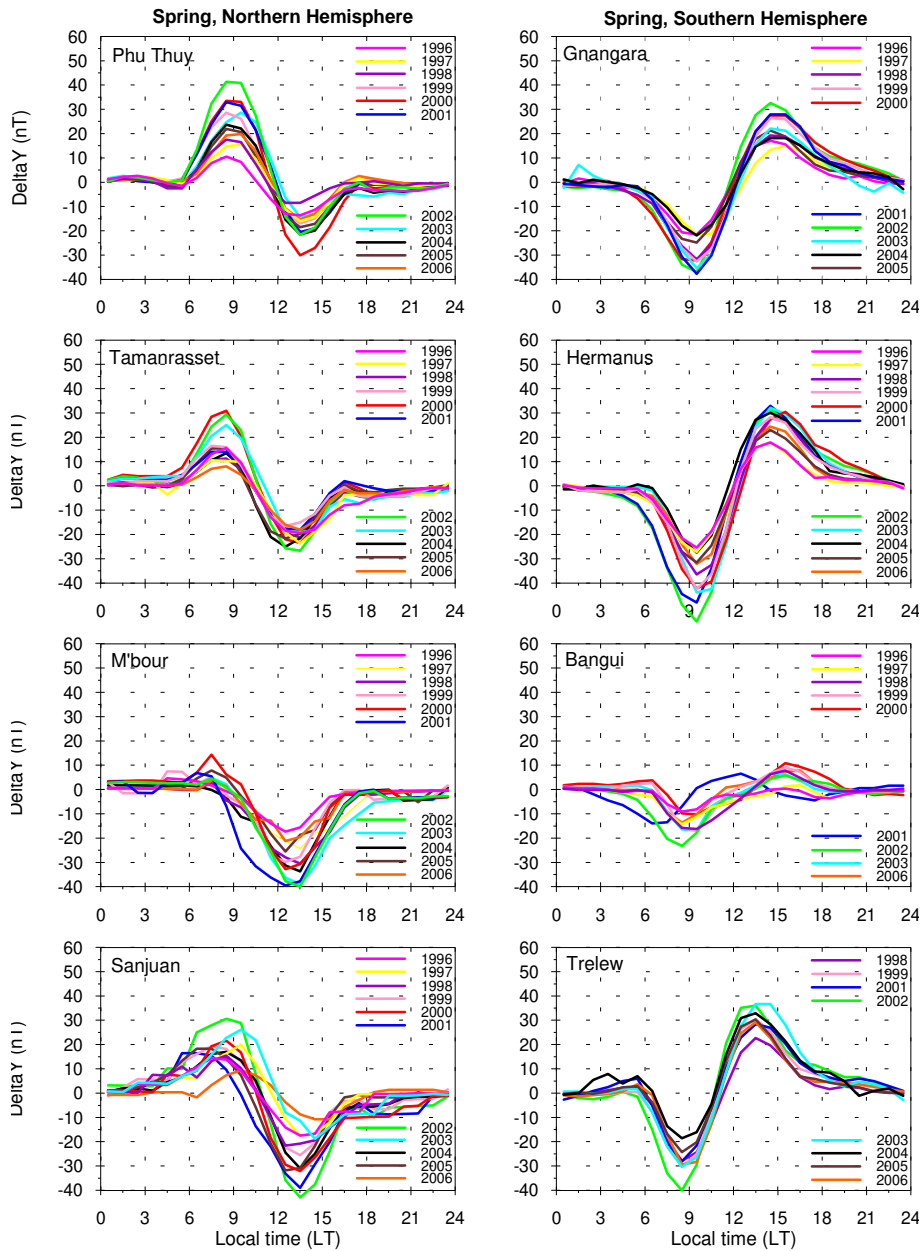
Fig. 11. Seasonal mean diurnal variations of the Y-component during Spring at Phu Thuy, Gngangara, Tamnarrasset, Hermanus, M’Bour, Bangui, San Juan and Trelew from 1996 to 2006 and during quiet magnetic time am <20 nT.
