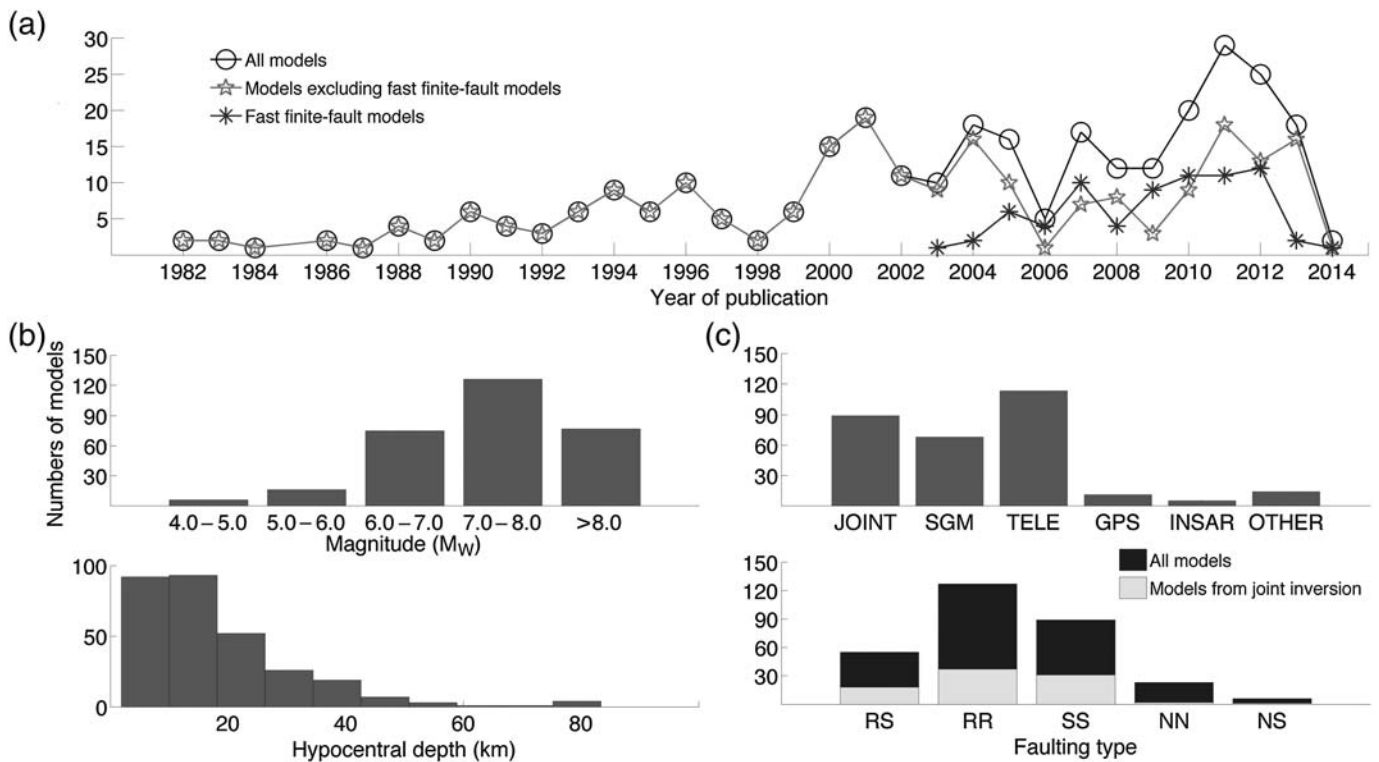
▲ Figure 4. The distribution of available rupture models in the SRCMOD database (status as of 30 June 2014): (a) time line of the number of rupture models published in the literature, (b) histograms of earthquake magnitudes (top) and hypocentral depths (bottom; two models for the 2013 Okhotsk Sea earthquake with the depth > 600 km are excluded), and (c) types of data used in the inversions (top) and faulting types of earthquakes in the database (bottom). JOINT, more than one data set is used for the inversion; SGM, strong ground-motion data; TELE, teleseismic recordings; GPS, Global Positioning System data; INSAR, Interferometric Synthetic Aperture Radar data; and OTHER, includes tsunami waveforms, leveling, trilateration, or other geophysical data. There are five different faulting styles: RS, reverse faulting with strike-slip components (or vice versa); RR, reverse faulting; SS, strike-slip faulting; NN, normal faulting; and NS, normal faulting with strike-slip components (or vice versa).
