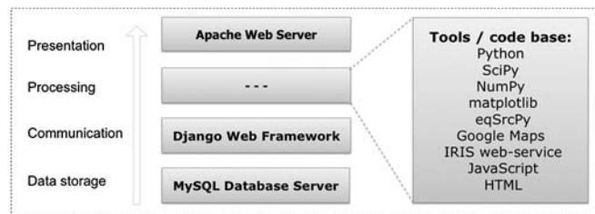
▲ Figure 1. A schematic description of components and software for the web development of the SRCMOD database.
