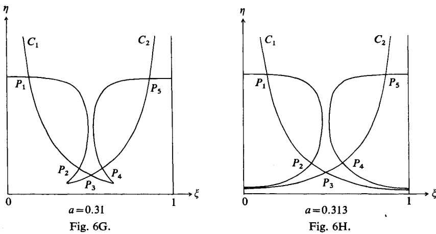
Fig. 6. Graphs of C_1 and C_2 , where each intersecting point P_i corresponds to a stationary solution of (SP).
