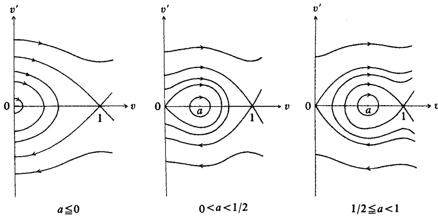
Fig. 1. Phase portraits for (v, v')
