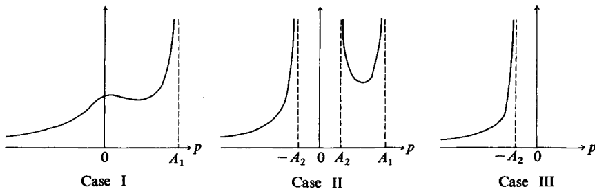
Fig. 2. Graphs of time mapping T_1
