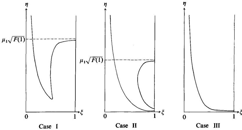
Fig. 3. Graphs of C_1
