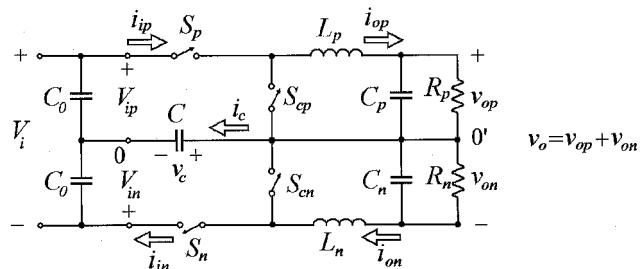
Fig. 1. Resonant buck converter R_p = R_n ; C_p = C_n .
