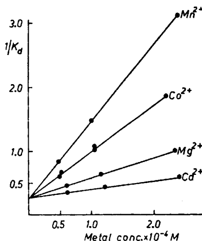
Fig. 1. Complex formation (1:1) of ATP with divalent metals. Determination by anion exchange resin method. See text for experimental conditions.
