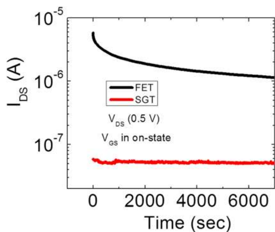
Figure 7. The drain current through the SGT and FET devices during the continuous stress applied for more than 100 min.
