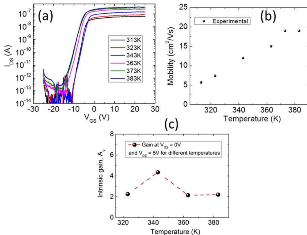
Figure 9. Temperature dependent transfer characteristics of ZnO NS-SGT device: (a) I_{DS} - V_{GS} curve of the SGT device at V_{DS} = 1 V for various temperatures, (b) Mobility versus temperature plot shows increase in mobility with temperature for SGT device, and (c) temperature dependent intrinsic gain.
