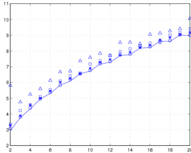
Figure 1: Lebesgue constant of Padua points (solid line) compared to that of the perturbed points with \alpha = 0.5 (circles), \alpha = 1 (asterisks), \alpha = 2 (squares), \alpha = 4 (triangles).
