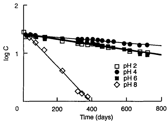
FIG. 2. Relationship between acetyl content and time over a pH range of 2 to 8 at 50 C for aspen.
