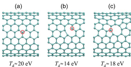
FIG. 5. (Color online) The atomic network of a (8,8) armchair nanotube and the energies needed to knock out the atom (marked with a circle) from the intact tube (a), nanotube with a vacancy (b), and a double vacancy (c).
