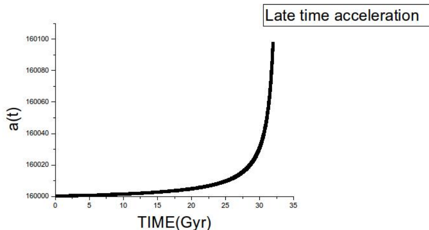
Figure 6. The scale factor ( a ) for late time acceleration era of expansion history as a function of t where t is age of universe. In this plot, we choose t_{\text{late}} = .4 Gyr, t_{\text{rip}} = 33 Gyr, T_{\text{late}} = 10^4 and T_{\text{end}} = 0 .
