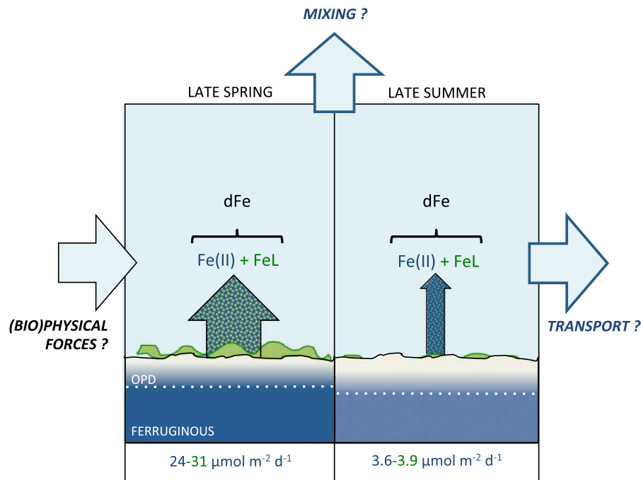
Fig. 10 Seasonal diffusive \text{Fe(II)} fluxes from the Celtic Sea Shelf and the proposed influence of stabilizing ligands. Calculated fluxes of \text{Fe(II)} to bottom water are indicated by arrow widths, and the potential influence of \text{Fe(II)} -stabilizing ligands by the density of green shading within arrows. Diffusive fluxes of \text{Fe(II)} which ignore the influence of ligands are smaller and correspond to minimum flux values described for each season. A shoaling of the oxygen penetration depth (OPD), increase in the surface porewater inventory of d\text{Fe(II)} and an increase in the diffusive flux of d\text{Fe(II)} to bottom waters coincides with the enhanced supply and decomposition of phytodetritus at the seafloor in late spring. An apparent 10–20 fold reduction in \text{Fe(II)} oxidation rates over empirical
