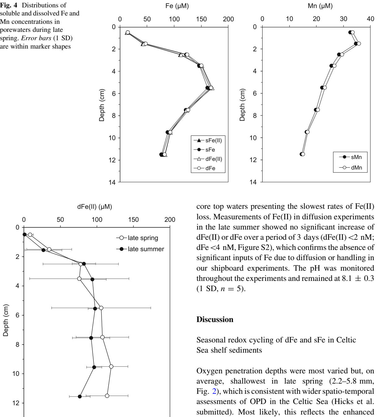
Fig. 5 Average porewater dFe(II) concentrations during late spring and late summer. Averages are from three measurements of replicate sediment cores and error bars are the standard deviation of these three measurements, dominantly reflecting natural heterogeneity within the sediment. Between seasons porewater dFe(II) concentrations are indistinguishable from natural heterogeneity below 1 cm depth. However, during late spring, above 1 cm depth dFe(II) concentrations are significantly higher than during the late summer
