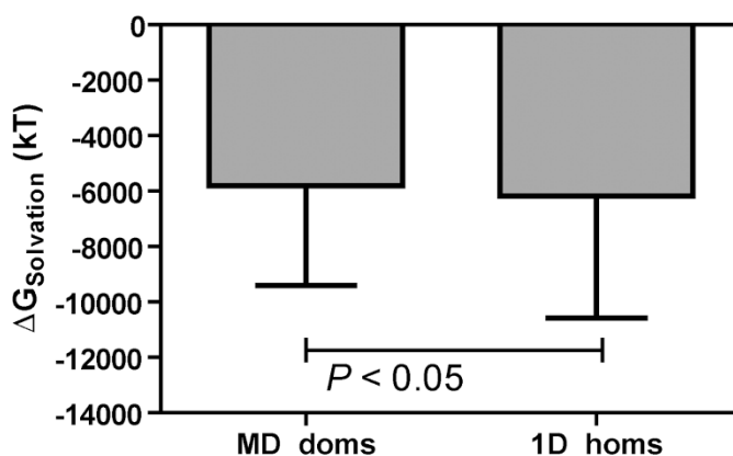
Figure 4 | Free energy of solvation of domains of multi-domain proteins and single domain homologues. The solvation free energy computed as the difference in the reaction field energy (See methods) of the protein when the external dielectric is changed from \epsilon=1 (air/vacuum) to \epsilon=80 (water) using the Delphi solvation model. The figure shows that the MD_doms have significantly higher solvation free energy in comparison to their single domain homologues (Paired t -test ; t = 2.262 , df = 704 , P = 0.0240 ).
