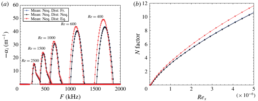
FIGURE 14. (Colour online) (a) Stability diagrams for Ma = 5 , T_e^* = T_{v,e}^* = 1500 K and P_e^* = 20 kPa. (a) Three different models of the disturbances: frozen, non-equilibrium and equilibrium. Mean flow is non-equilibrium. (b) The N factor diagram corresponding to (a). Only 2D waves with \beta = 0 are included.
