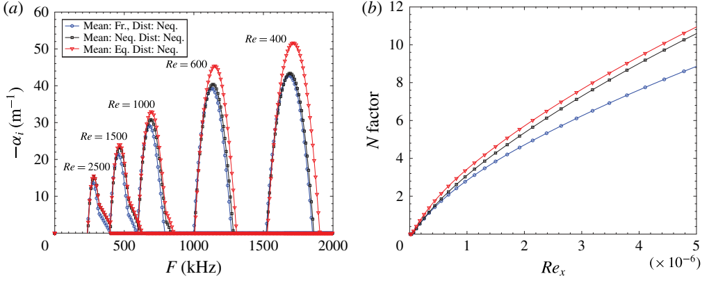
FIGURE 13. (Colour online) (a) Stability diagrams for Ma = 5 , T_e^* = T_{v,e}^* = 1500 K and P_e^* = 20 kPa. Three different models of the mean flow: frozen, non-equilibrium and equilibrium. Disturbances are non-equilibrium. (b) The N factor diagram corresponding to (a). Only 2D waves with \beta = 0 are included.
