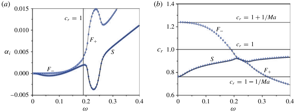
FIGURE 2. (Colour online) Comparison of present stability analysis (symbols) with the results of Fedorov & Tumin ( \square ) (solid lines). Flow is a perfect gas with Ma = 4.2 , T_o^* = 300 K, Re = 2000 , adiabatic wall. Waves are 2D with \beta = 0 ; (a) growth rates; (b) phase speeds.
