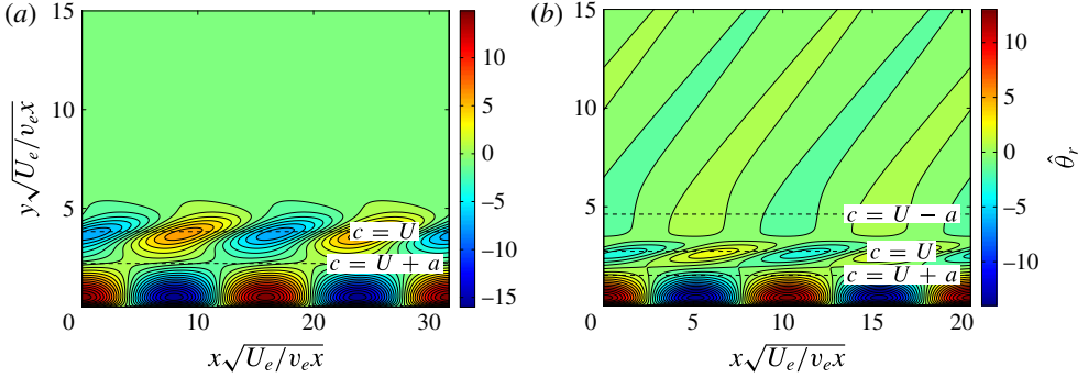
FIGURE 9. (Colour online) Contours of temperature fluctuations at two points along the dispersion curve in figure \Gamma for Re = 2000 , T_e^* = 1500 K, T_w^* = 300 K, Ma = 5 : (a) \omega = 0.35 , subsonic mode; (b) \omega = 0.45 , supersonic mode.
