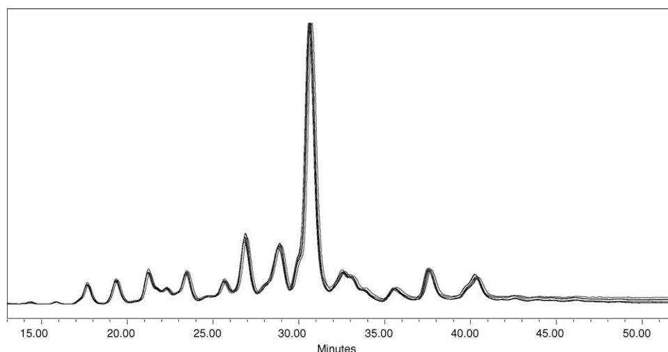
Fig. 2. Overlay of seven N -glycan chromatograms from plasma samples from the same individual on seven occasions during 5 days. Glycans were released from proteins, labeled and separated using hydrophilic interaction high-performance liquid chromatography.
