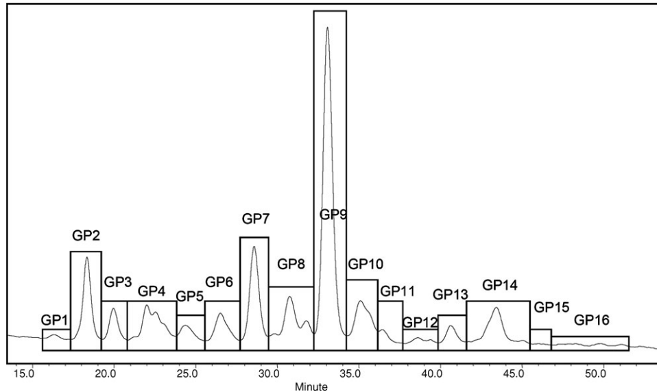
Fig. 1. N -Glycan profile from the human plasma sample divided into 16 groups of glycans. The glycan structures present in each group correspond to those given in Table I. Glycans were released from proteins, labeled and separated using hydrophilic interaction high-performance liquid chromatography.
