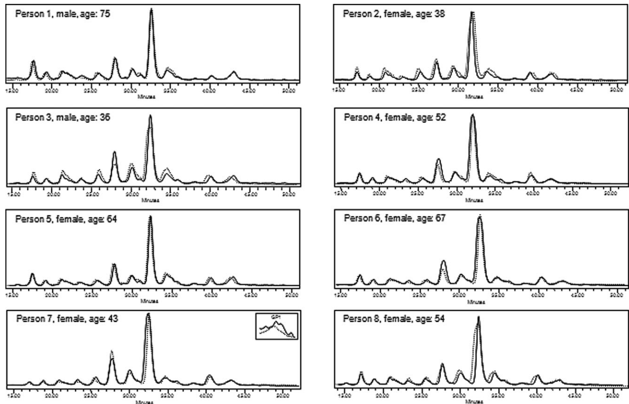
Fig. 3. N -Glycan HPLC profiles from eight individuals that were sampled twice with an interval of approximately 1 year. Glycans were released from proteins, labeled and separated using hydrophilic interaction high-performance liquid chromatography. In general, glycan patterns in most of the individuals did not change significantly after a year, but some glycans in some individuals did change considerably. The largest observed change was a nearly 40% increase in GP1 that was observed in person 7.
