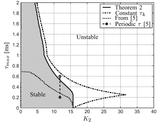
Fig. 5. Stability region in terms of K_2 and time-varying delays \tau_k \in [0, \tau_{\max}] (for h = 1 \text{ ms} , K_1 = 50 ) for Theorem 2, based on [5], and for constant delays equal to \tau_{\max} .
