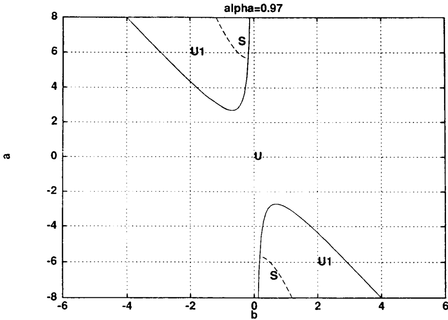
FIG. 3(g). Region of FW stability in the (b, a) plane for a single complex Ginzburg-Landau equation; \alpha = 0.97 .
