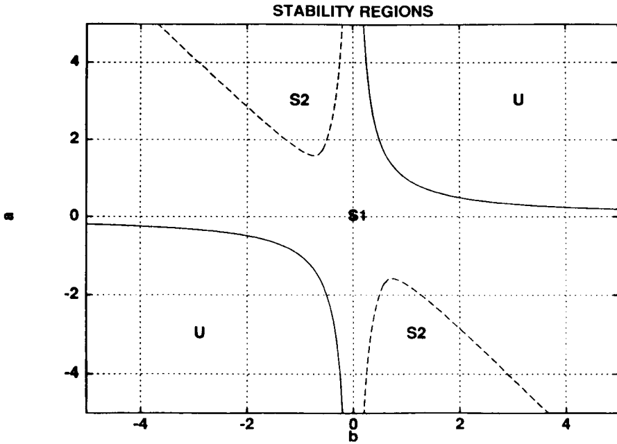
FIG. 4. Regions of stability in the (b, a) plane for a single complex Ginzburg-Landau equation.
