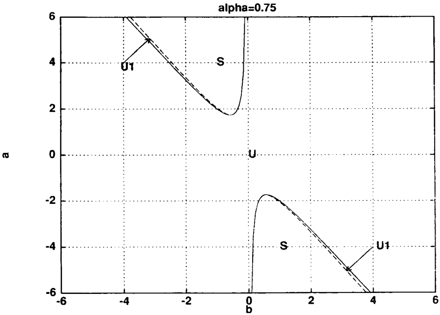
FIG. 3(b). Region of FW stability in the (b, a) plane for a single complex Ginzburg-Landau equation; \alpha = 0.75 .
