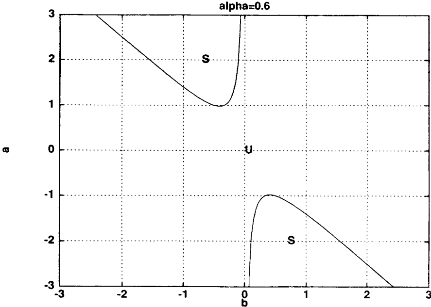
FIG. 1(c). Region of LW stability in the (b, a) plane for a single complex Ginzburg-Landau equation; \alpha = 0.6 .
