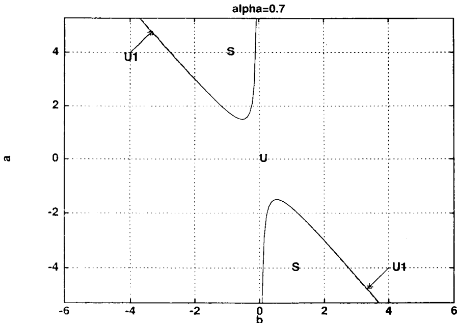
FIG. 3(a). Region of FW stability in the (b, a) plane for a single complex Ginzburg-Landau equation; \alpha = 0.7 .
