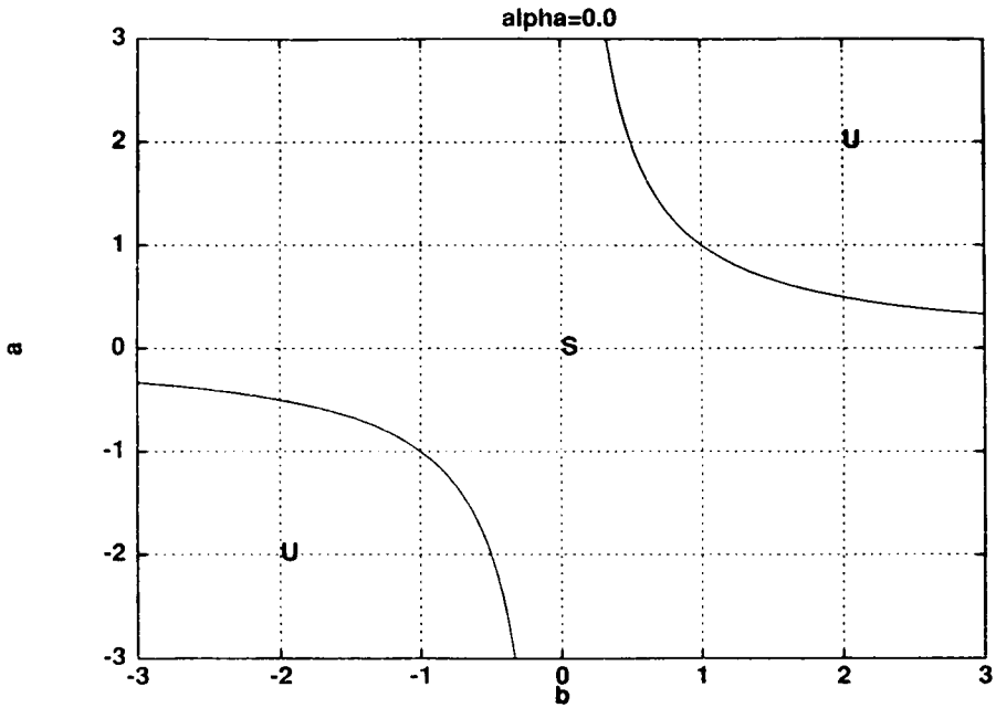
FIG. 1(a). Region of LW stability in the (b, a) plane for a single complex Ginzburg-Landau equation; \alpha = 0 .
