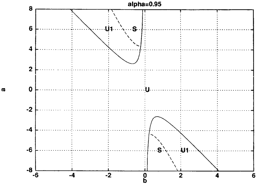
FIG. 3(f). Region of FW stability in the (b, a) plane for a single complex Ginzburg-Landau equation; \alpha = 0.95 .
