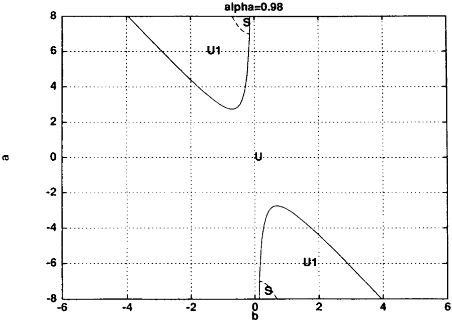
FIG. 3(h). Region of FW stability in the (b, a) plane for a single complex Ginzburg-Landau equation; \alpha = 0.98 .
