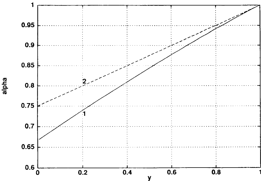
FIG. 2. Ranges of variation of y in the parametric dependence (2.17)–(2.20). For a fixed \alpha ( \frac{2}{3} < \alpha < \frac{3}{4} ), y varies between zero and y^* (see (2.23)), and between 4\alpha - 3 and y^* for \frac{3}{4} < \alpha < 1 .
