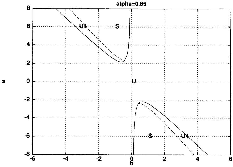
FIG. 3(d). Region of FW stability in the (b, a) plane for a single complex Ginzburg-Landau equation; \alpha = 0.85 .
