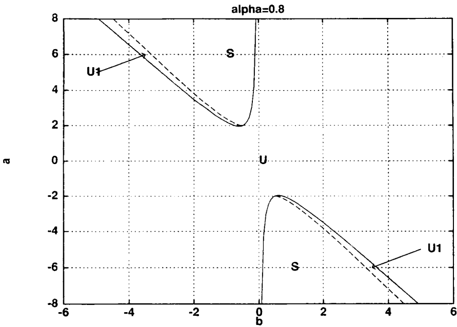
FIG. 3(c). Region of FW stability in the (b, a) plane for a single complex Ginzburg-Landau equation; \alpha = 0.8 .
