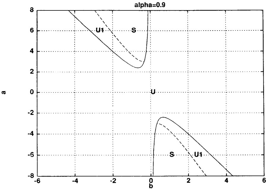
FIG. 3(e). Region of FW stability in the (b, a) plane for a single complex Ginzburg-Landau equation; \alpha = 0.9 .
