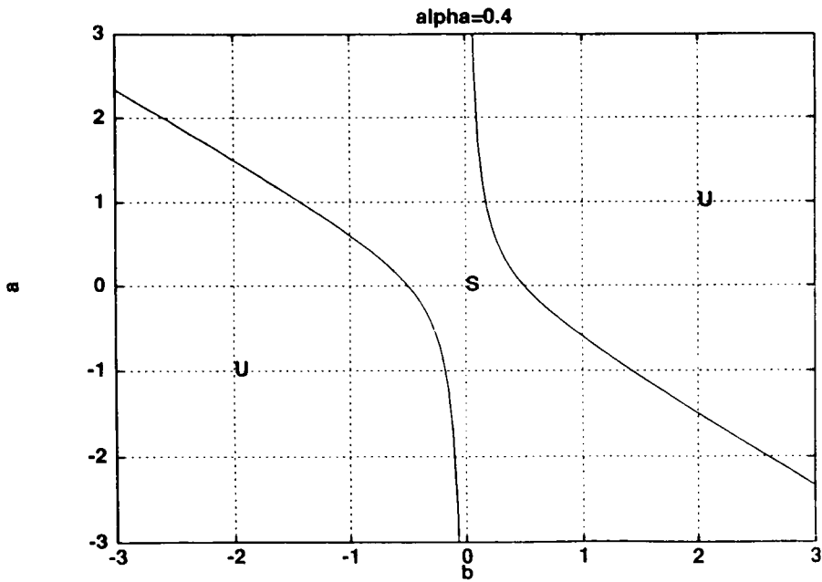
FIG. 1(b). Region of LW stability in the (b, a) plane for a single complex Ginzburg-Landau equation; \alpha = 0.4 .
