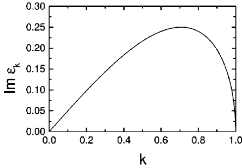
FIG. 2. Imaginary part of the excitation energy (in units of \mu ) vs the transverse momentum k (in units of l^{-1} ) for a kinkwise condensate in the absence of a trapping field.
