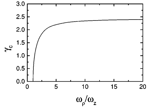
FIG. 3. Critical parameter \gamma_c vs the aspect ratio for a kinkwise condensate in a cylindrical trap.
