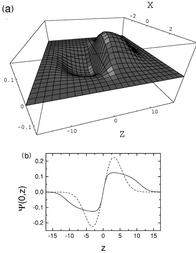
FIG. 1. Condensate wave function \Psi_0 of a kinkwise state in a cylindrical trap for the ratio of the mean-field interaction at maximum density ( n_{0m} ) to the trap frequencies, n_{0m}\bar{U}:\hbar\omega_\rho:\hbar\omega_z = 10:10:1 ( \bar{U} = 4\pi\hbar^2 a/m , a > 0 is the scattering length, and m the atom mass). The axial ( z ) and radial ( x ) coordinates are given in units of the correlation length l = \hbar/\sqrt{n_{0m}\bar{U}} , and (normalized to unity) \Psi_0 in units of l^{-3/2} . In (b) the solid curve is \Psi_0(0,z) and the dashed curve is the first (axially) excited state of a harmonic oscillator.
