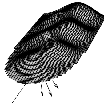
FIG. 5. A mechanism of instability leading to undulations in a finger of delamination: longitudinal buckling in the tail of the blister breaks the symmetry at the tip, and favors oblique propagation.
