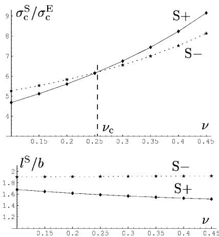
FIG. 3. Critical compression, \sigma_c^S , and wavelength, l^S , of the mode destabilizing the Euler column, by symmetric ( S^+ ) or antisymmetric ( S^- ) secondary buckling. Dependence on the Poisson ratio of the film, \nu is plotted.
