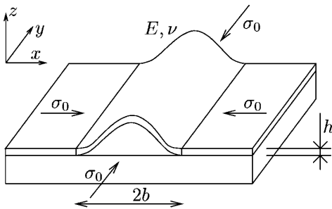
FIG. 1. The Euler column, solution of the FvK equations above the critical initial compression \sigma_0 > \sigma_c^E .
