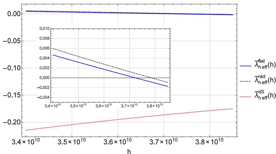
Figure 10. The effective quartic Higgs coupling, as defined by the relation \bar{\lambda}_{\text{Higgs}}(h) \equiv \frac{4V^{(1)}(h)}{h^4} , for various equations of state: flat — flat spacetime result, rad — radiation dominance ( p = \frac{1}{3}\rho ), dS — de Sitter like ( p = -\rho ). The energy density was given by \rho = \rho_{hc} + (\frac{y_t h}{\sqrt{2}})^4 , where \rho_{hc} was specified by the relation (4.36) and equal to \rho_{hc} = (2.04 \cdot 10^{14} \text{GeV})^4 . The X field was constant and set as equal to X = v_X . The non-minimal couplings were \xi_h = \xi_X = 0 at the \mu = m_t . The insert shows a close up of the difference between the flat spacetime and the radiation dominated era.
