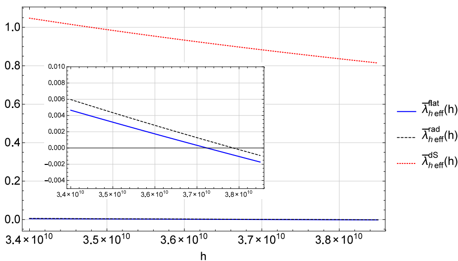
Figure 11. The effective quartic Higgs coupling, as defined by the relation \bar{\lambda}_{\text{Higgs}}(h) \equiv \frac{4V^{(1)}(h)}{h^4} , for various equations of state: flat — flat spacetime result, rad — radiation dominance ( p = \frac{1}{3}\rho ), dS — de Sitter like ( p = -\rho ). The energy density was given by \rho = \rho_{hc} + (\frac{y_t h}{\sqrt{2}})^4 , where \rho_{hc} was specified by the relation (4.36) and equal to \rho_{hc} = (2.04 \cdot 10^{14} \text{GeV})^4 . The X field was constant and set as equal to X = v_X . The non-minimal couplings were \xi_h = \xi_X = \frac{1}{3} at the \mu = m_t . The insert shows a close up of the difference between the flat spacetime and the radiation dominated era.
