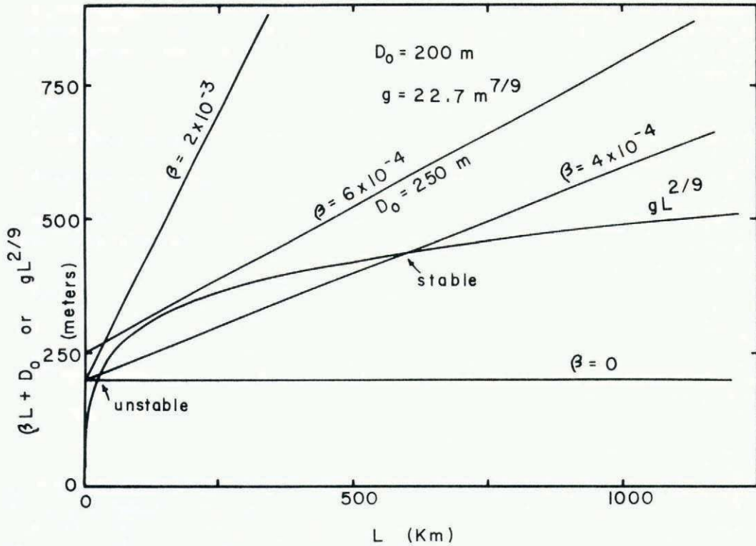
Fig. 4. Plots of the functions gL^{2/9} and (\beta L + D_0) versus L . Curves plotted for g = 22.7 \text{ m}^{7/9} , D_0 = 200 \text{ m} and (for one curve) 250 \text{ m} , and \beta = 2 \times 10^{-3} , 6 \times 10^{-4} , 4 \times 10^{-4} and 0 . Values of L for steady-state ice sheets occur where the curves of gL^{2/9} and (\beta L + D_0) cross.
