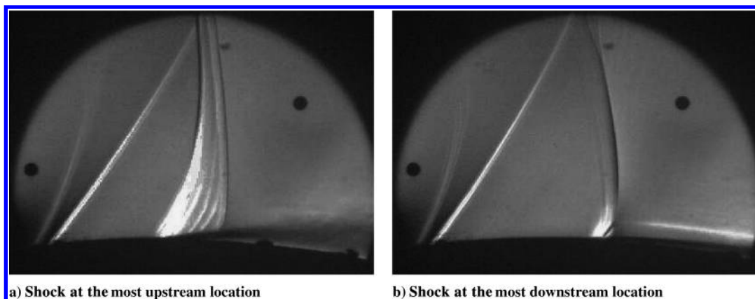
Fig. 2 Instantaneous schlieren images from Jacquin et al. [22].
