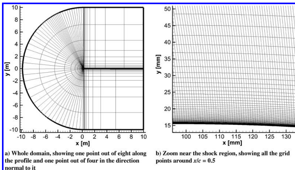
Fig. 4 Reference mesh used for the numerical simulation and for the stability analysis.
