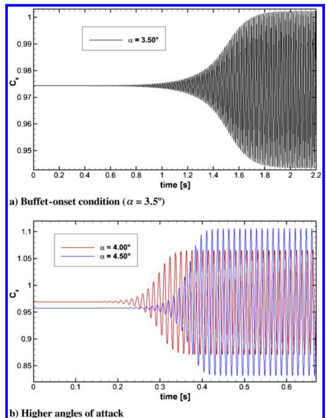
Fig. 10 Evolution of lift coefficient in URANS solutions for different angles of attack.
