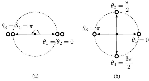
Fig. 1. Phase synchronization and balancing examples for N = 4 . (a) Phase arrangement is balanced modulo 2\pi and synchronized modulo \pi ; i.e., p_\theta = 0 and 2|p_{2\theta}| = 1 . (b) Phase arrangement is balanced modulo 2\pi , balanced modulo \pi , and synchronized modulo \pi/2 ; i.e., p_\theta = p_{2\theta} = 0 and 4|p_{4\theta}| = 1 .
