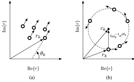
Fig. 2. Synchronizing the state variables s_k = -i\omega_0 c_k . (a) If \omega_0 = 0 , then synchronization of s_k generates a parallel formation. (b) If \omega_0 \neq 0 , then synchronization of s_k generates a circular formation centered at c_k = r_k + i\omega_0^{-1} e^{i\theta_k} .
