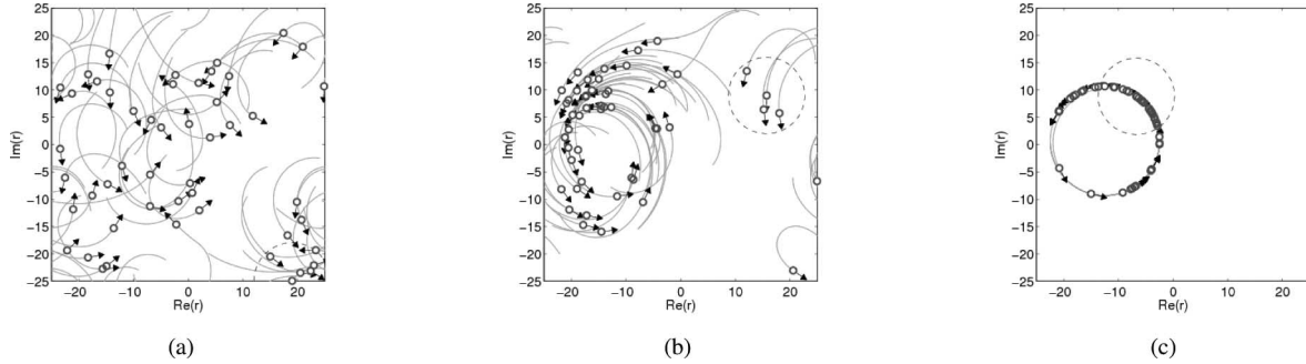
Fig. 4. Snapshots after 20, 75, and 250 time steps of simulation results for N = 50 particles randomly initialized in a 50 by 50 spatial domain with periodic boundary conditions. The particles are subject to the dynamic control (21) with K = -0.1 and a time-varying zonal sensory graph G(t) . The radius of proximity \rho_k = 7 for all particles is depicted, for a single particle, as a dashed circle. Setting \omega_0 = 0.1 stabilizes circular motion with radius \rho_0 = |\omega_0^{-1}| ; setting \omega_0 = 0 stabilizes a parallel motion (not shown). (a) t = 20 . (b) t = 75 . (c) t = 250 .
