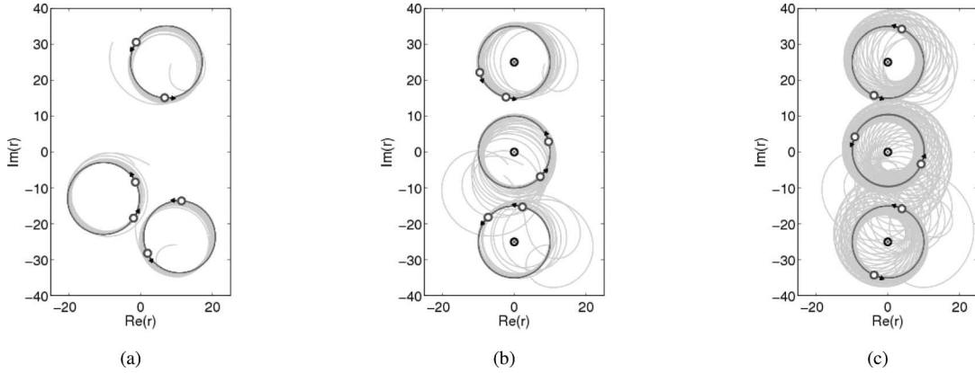
Fig. 3. Simulation results of (1) subject to Laplacian control with separate spacing and phase graphs with reference particles and nested phase potentials. (a) Control (38) with M = N = 6 , B = 3 , and K = \omega_0 = 0.1 stabilizes three separate circular formations of radius \rho_0 = |\omega_0^{-1}| and a splay arrangement of all 6 particle phases. (b) Control (39) fixes the centers of the circular formations to the reference locations c_0^{(b)} = i25(b-2) , b = 1, 2, 3 denoted by crossed circles. (c) Control (40) stabilizes a nested (M, N) -pattern with Q = 3 and M = N = (2, 4, 4)^T . Trajectories start from random initial conditions, and are plotted after elapsed time equivalent to 50 revolutions; the last revolution of each particle is plotted in dark gray.
