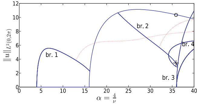
FIG. 10. Zoom in of Fig. 1(a) with \nu \in [0.1, 1] . Branches are labelled as used in Tables 4–6 in Section 4.2: Branch 1—unimodal steady states; branch 2—bimodal steady states; branch 3—trimodal steady states; branch 4—tetramodal steady states. The cross and open circle symbols indicate the steady states (stable and unstable, respectively) that are shown in the Fig. 8.
